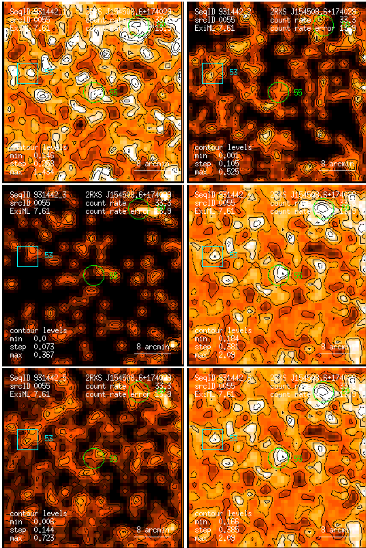
Figure 55: RASS 931442: detection 0055: band rate images, Gaussian filter: (1) PSPC channels 11 – 41, (2) 52 – 90, (3) 91 – 201, (4) 11 – 235, (5) 52 – 201, (6) 11 – 201. Broad band rates in counts/ks. Band rate contour levels in counts/ks/arcmin 2 .
