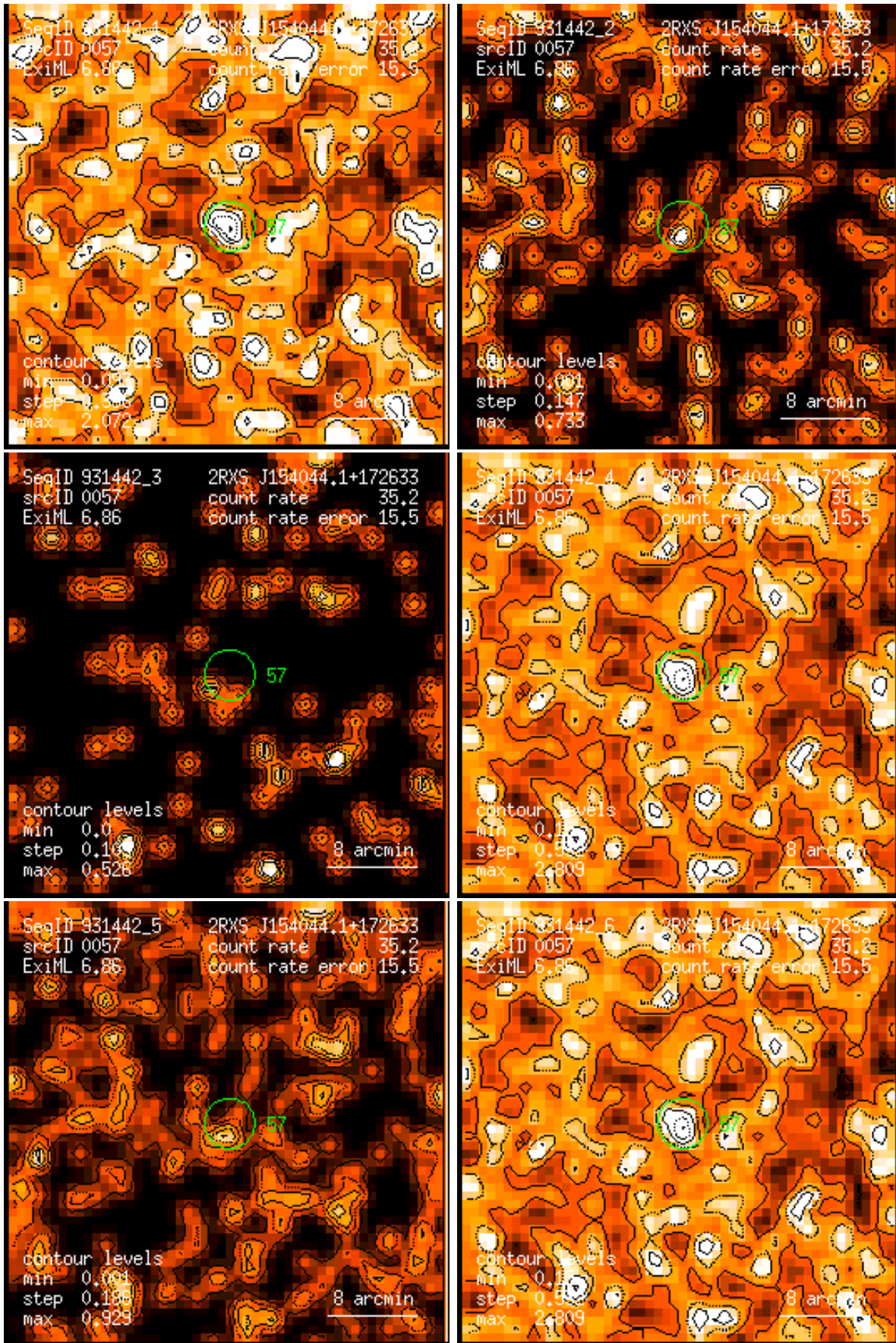
Figure 57: RASS 931442: detection 0057: band rate images, Gaussian filter: (1) PSPC channels 11 – 41, (2) 52 – 90, (3) 91 – 201, (4) 11 – 235, (5) 52 – 201, (6) 11 – 201. Broad band rates in counts/ks. Band rate contour levels in counts/ks/arcmin 2 .
