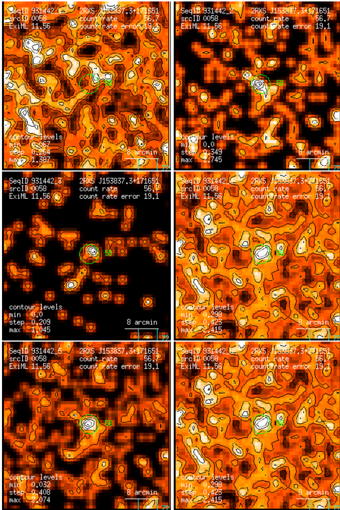
Figure 58: RASS 931442: detection 0058: band rate images, Gaussian filter: (1) PSPC channels 11 – 41, (2) 52 – 90, (3) 91 – 201, (4) 11 – 235, (5) 52 – 201, (6) 11 – 201. Broad band rates in counts/ks. Band rate contour levels in counts/ks/arcmin 2 .
