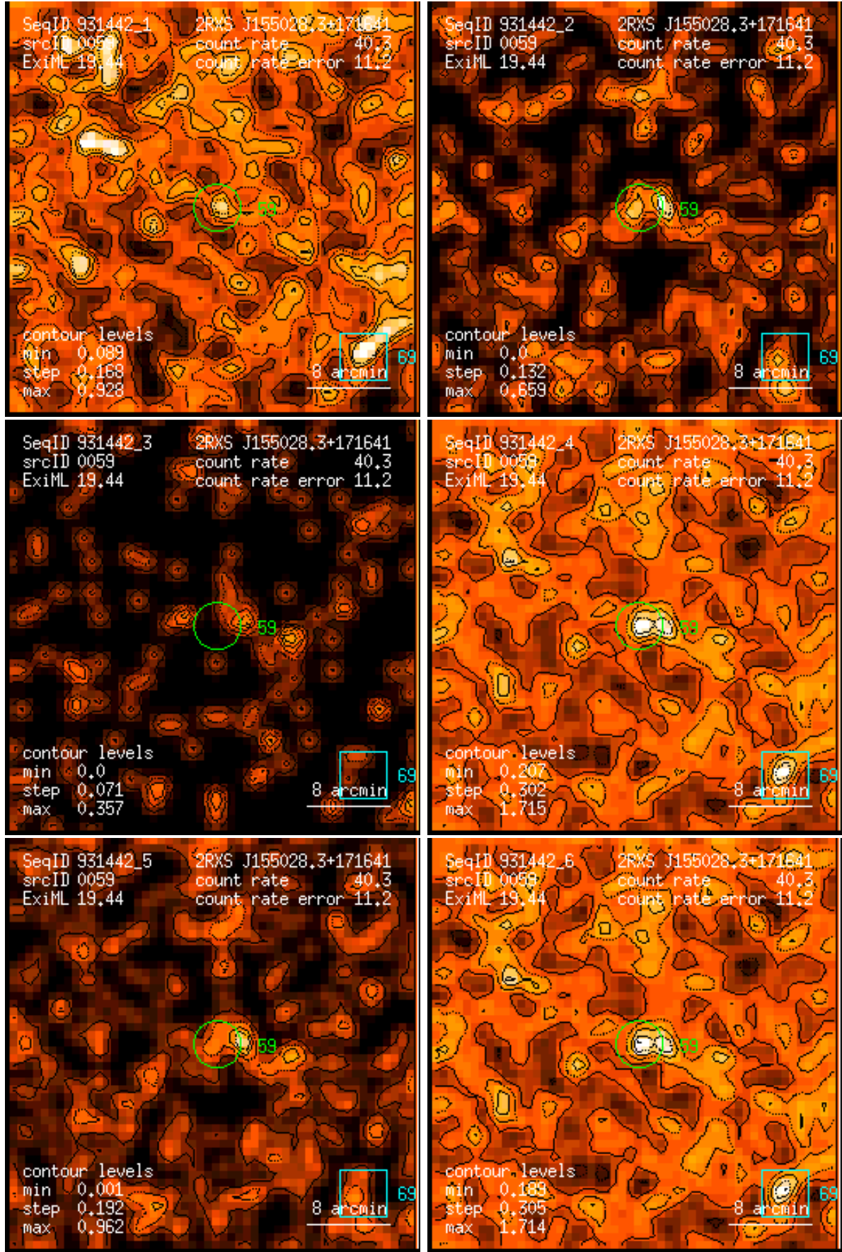
Figure 59: RASS 931442: detection 0059: band rate images, Gaussian filter: (1) PSPC channels 11 – 41, (2) 52 – 90, (3) 91 – 201, (4) 11 – 235, (5) 52 – 201, (6) 11 – 201. Broad band rates in counts/ks. Band rate contour levels in counts/ks/arcmin 2 .
