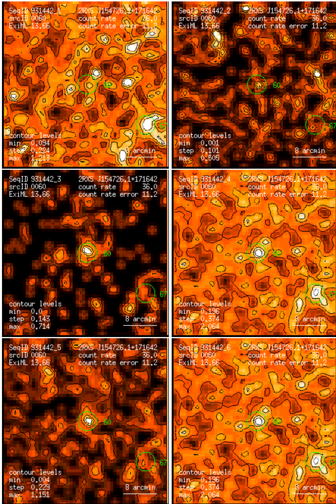
Figure 60: RASS 931442: detection 0060: band rate images, Gaussian filter: (1) PSPC channels 11 – 41, (2) 52 – 90, (3) 91 – 201, (4) 11 – 235, (5) 52 – 201, (6) 11 – 201. Broad band rates in counts/ks. Band rate contour levels in counts/ks/arcmin 2 .
