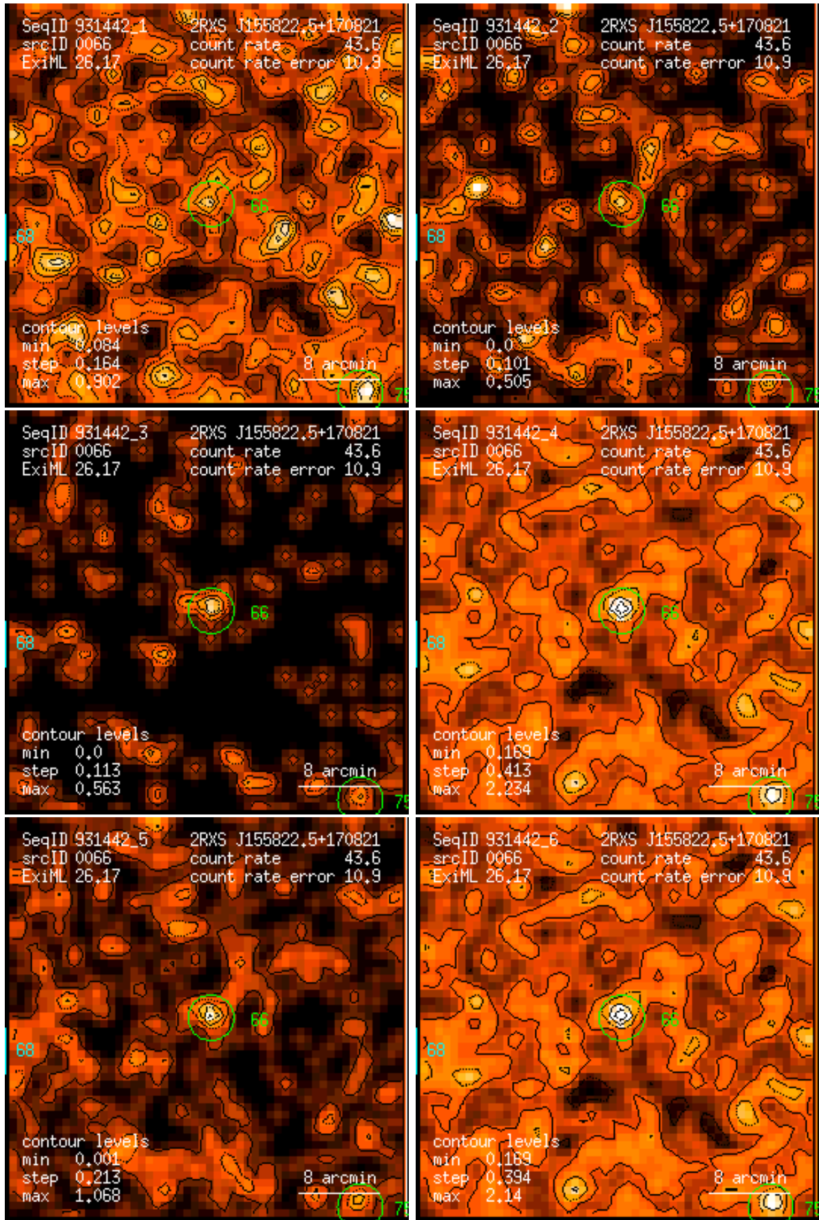
Figure 66: RASS 931442: detection 0066: band rate images, Gaussian filter: (1) PSPC channels 11 – 41, (2) 52 – 90, (3) 91 – 201, (4) 11 – 235, (5) 52 – 201, (6) 11 – 201. Broad band rates in counts/ks. Band rate contour levels in counts/ks/arcmin 2 .
