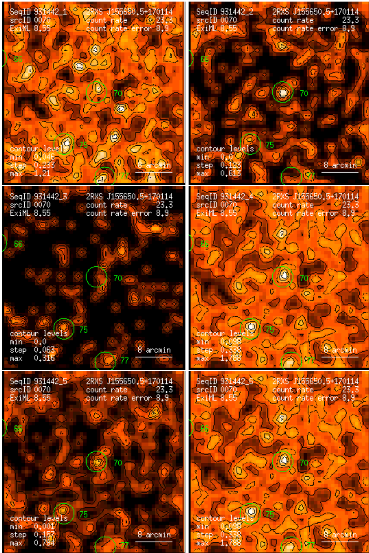
Figure 70: RASS 931442: detection 0070: band rate images, Gaussian filter: (1) PSPC channels 11 – 41, (2) 52 – 90, (3) 91 – 201, (4) 11 – 235, (5) 52 – 201, (6) 11 – 201. Broad band rates in counts/ks. Band rate contour levels in counts/ks/arcmin 2 .
