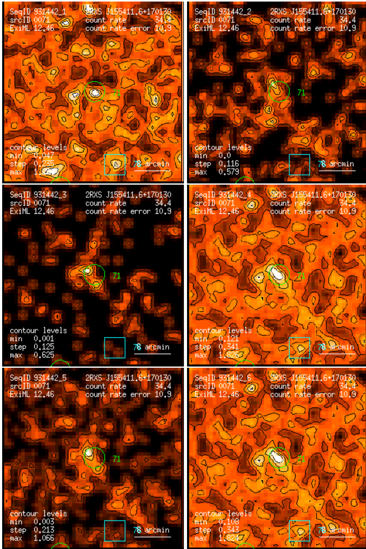
Figure 71: RASS 931442: detection 0071: band rate images, Gaussian filter: (1) PSPC channels 11 – 41, (2) 52 – 90, (3) 91 – 201, (4) 11 – 235, (5) 52 – 201, (6) 11 – 201. Broad band rates in counts/ks. Band rate contour levels in counts/ks/arcmin 2 .
