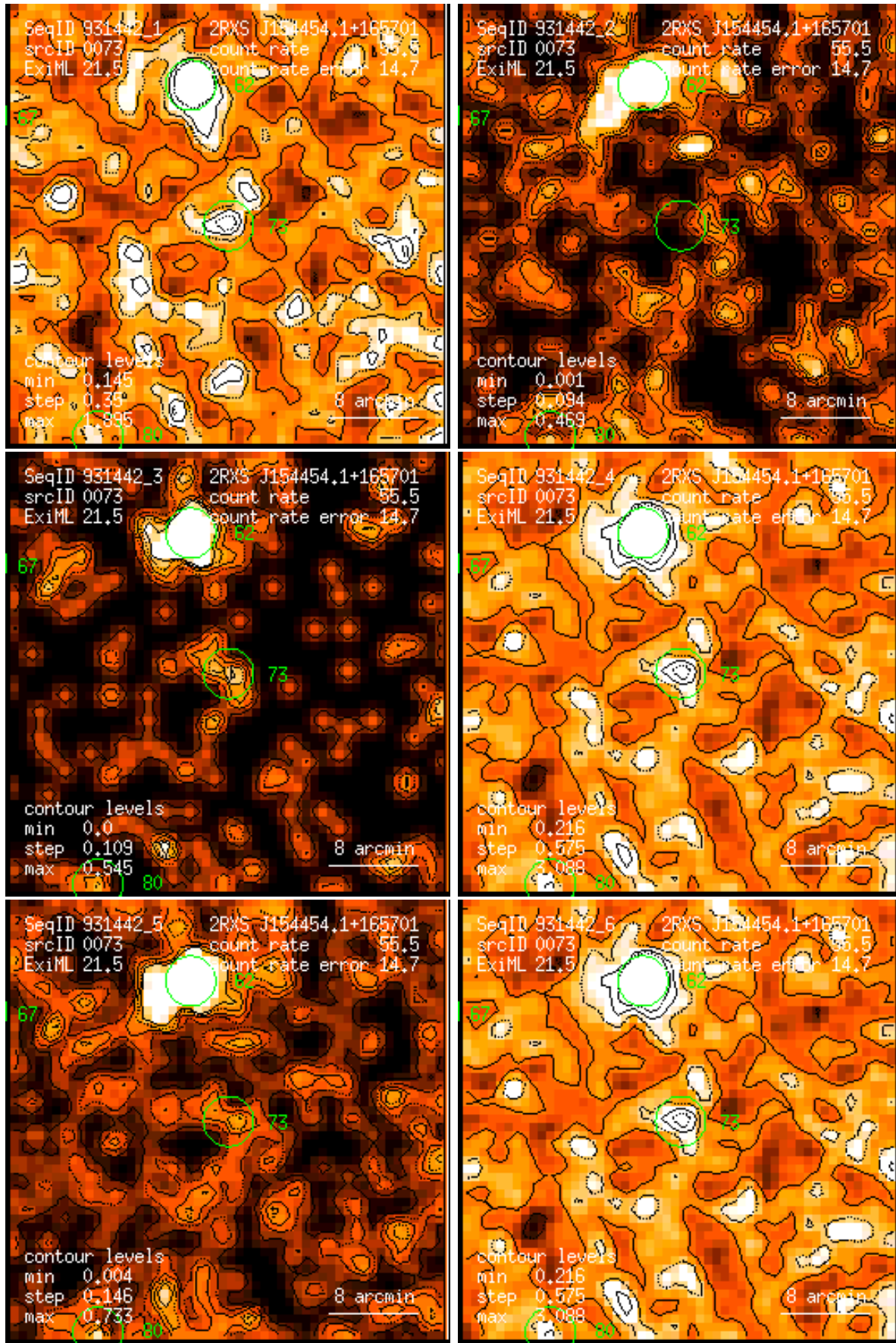
Figure 73: RASS 931442: detection 0073: band rate images, Gaussian filter: (1) PSPC channels 11 – 41, (2) 52 – 90, (3) 91 – 201, (4) 11 – 235, (5) 52 – 201, (6) 11 – 201. Broad band rates in counts/ks. Band rate contour levels in counts/ks/arcmin 2 .
