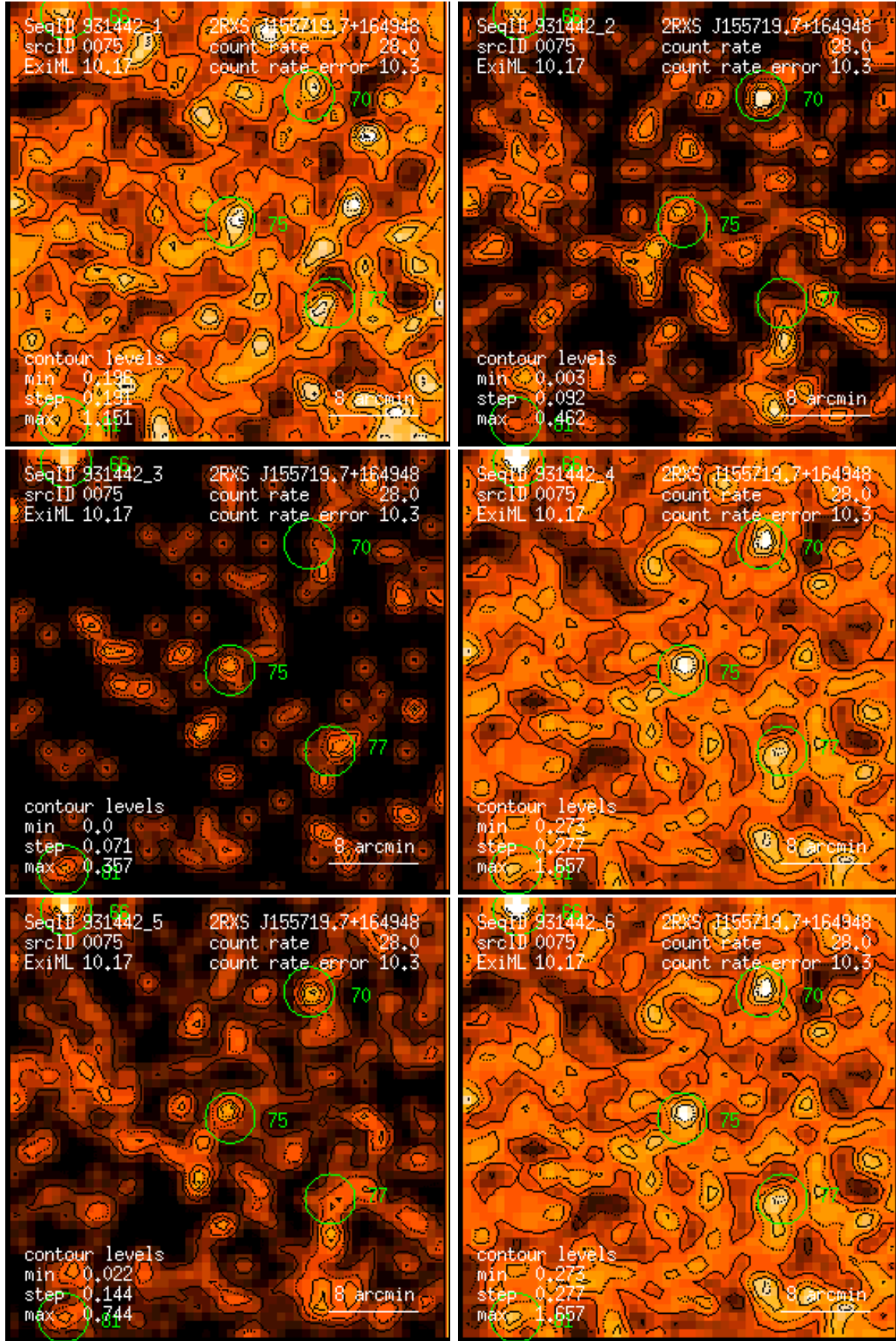
Figure 75: RASS 931442: detection 0075: band rate images, Gaussian filter: (1) PSPC channels 11 – 41, (2) 52 – 90, (3) 91 – 201, (4) 11 – 235, (5) 52 – 201, (6) 11 – 201. Broad band rates in counts/ks. Band rate contour levels in counts/ks/arcmin 2 .
