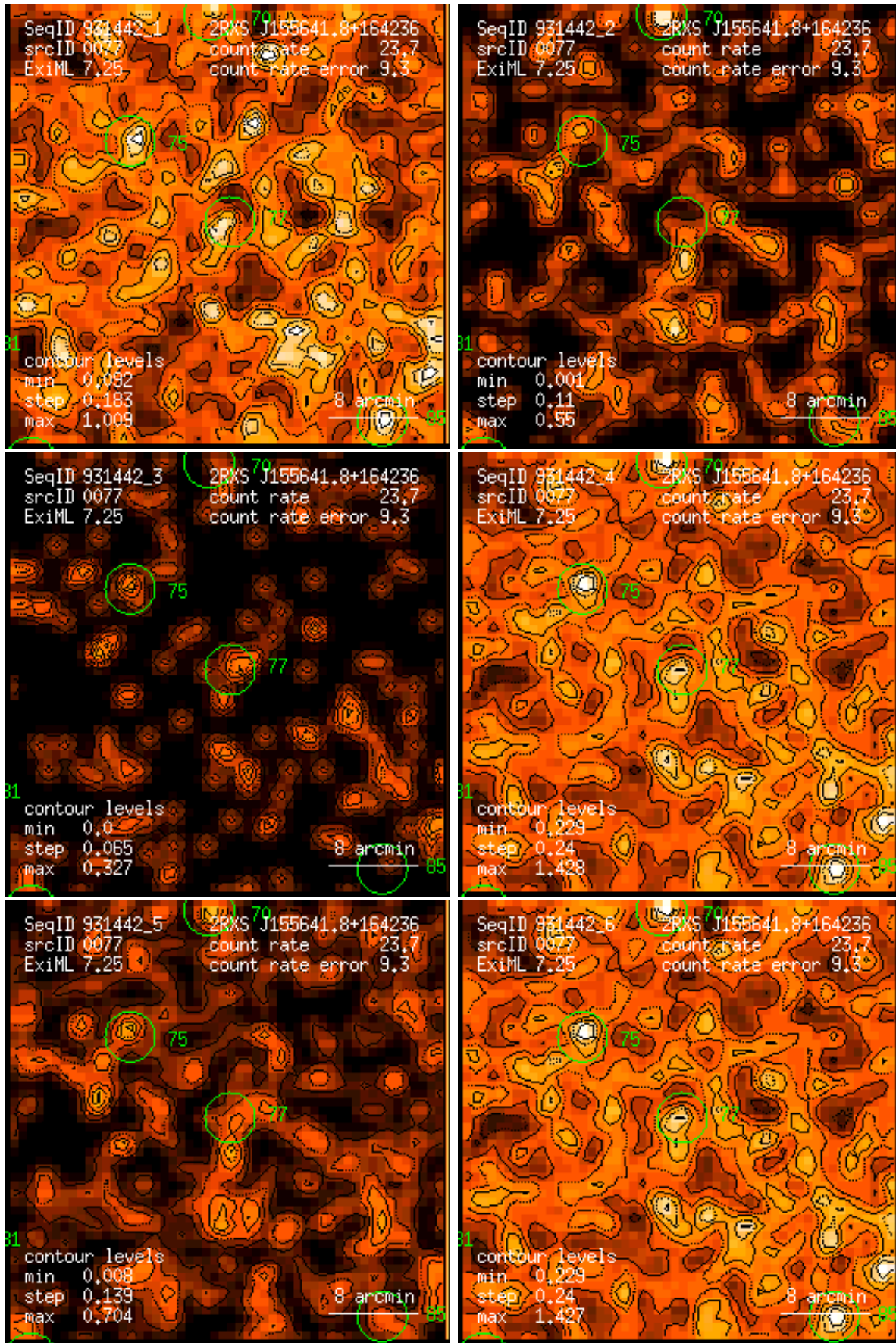
Figure 77: RASS 931442: detection 0077: band rate images, Gaussian filter: (1) PSPC channels 11 – 41, (2) 52 – 90, (3) 91 – 201, (4) 11 – 235, (5) 52 – 201, (6) 11 – 201. Broad band rates in counts/ks. Band rate contour levels in counts/ks/arcmin 2 .
