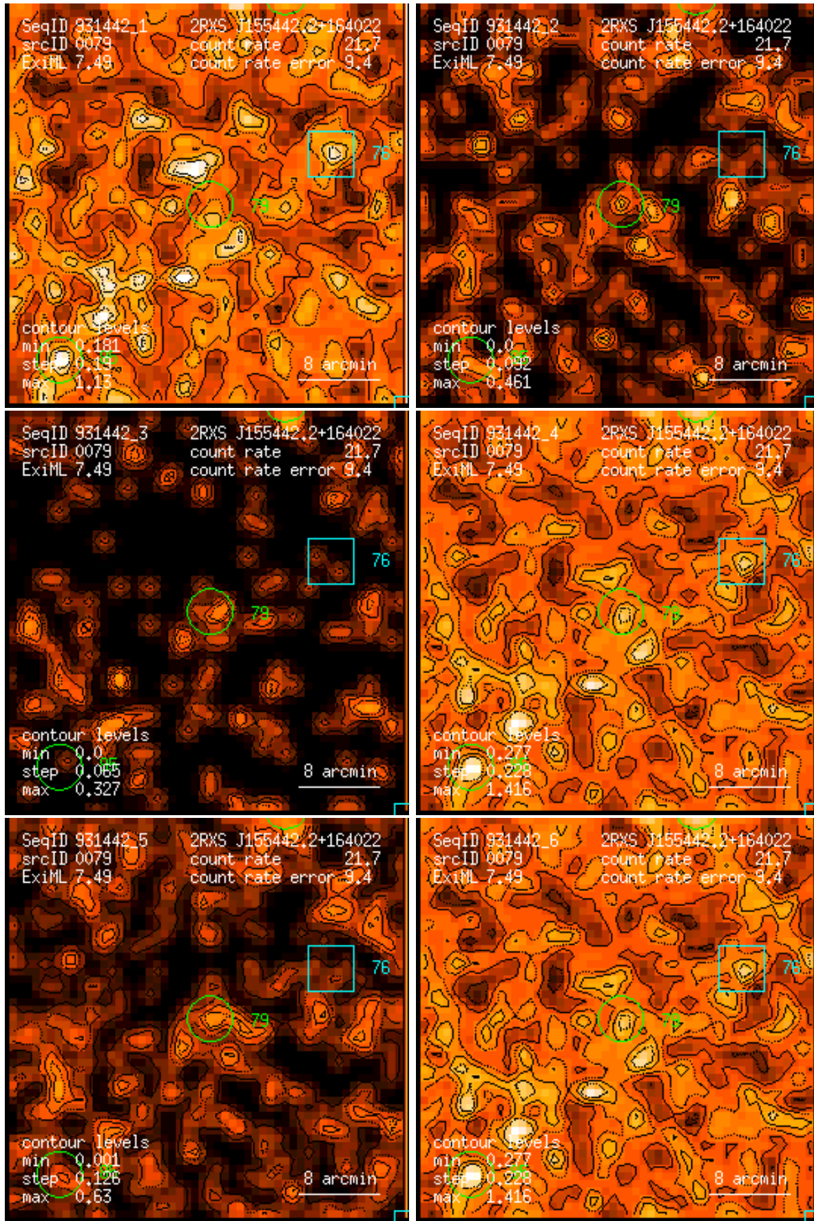
Figure 79: RASS 931442: detection 0079: band rate images, Gaussian filter: (1) PSPC channels 11 – 41, (2) 52 – 90, (3) 91 – 201, (4) 11 – 235, (5) 52 – 201, (6) 11 – 201. Broad band rates in counts/ks. Band rate contour levels in counts/ks/arcmin 2 .
