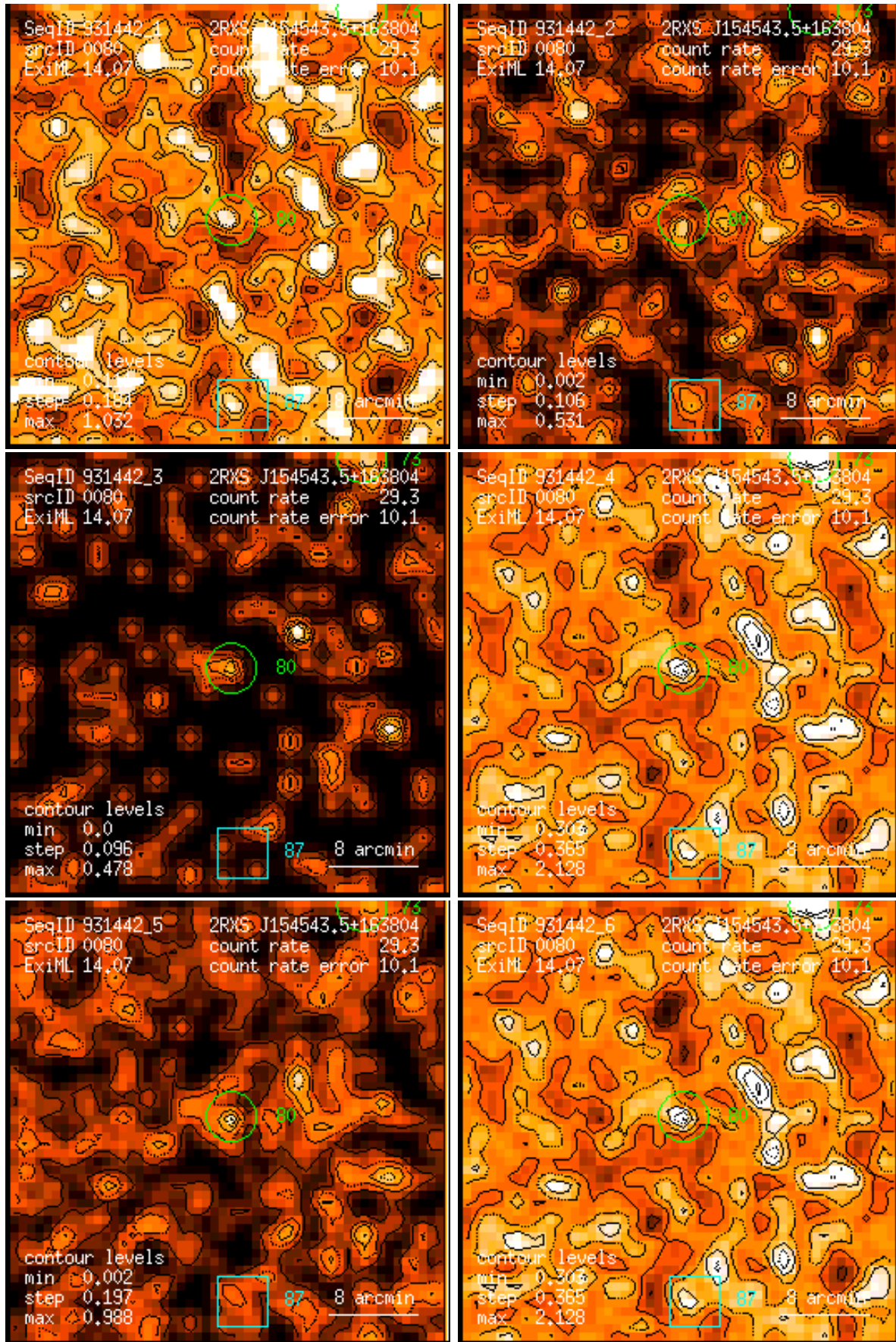
Figure 80: RASS 931442: detection 0080: band rate images, Gaussian filter: (1) PSPC channels 11 – 41, (2) 52 – 90, (3) 91 – 201, (4) 11 – 235, (5) 52 – 201, (6) 11 – 201. Broad band rates in counts/ks. Band rate contour levels in counts/ks/arcmin 2 .
