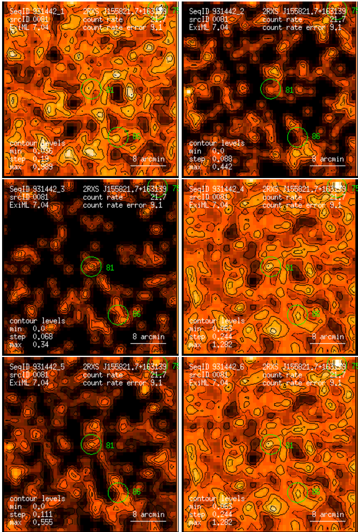
Figure 81: RASS 931442: detection 0081: band rate images, Gaussian filter: (1) PSPC channels 11 – 41, (2) 52 – 90, (3) 91 – 201, (4) 11 – 235, (5) 52 – 201, (6) 11 – 201. Broad band rates in counts/ks. Band rate contour levels in counts/ks/arcmin 2 .
