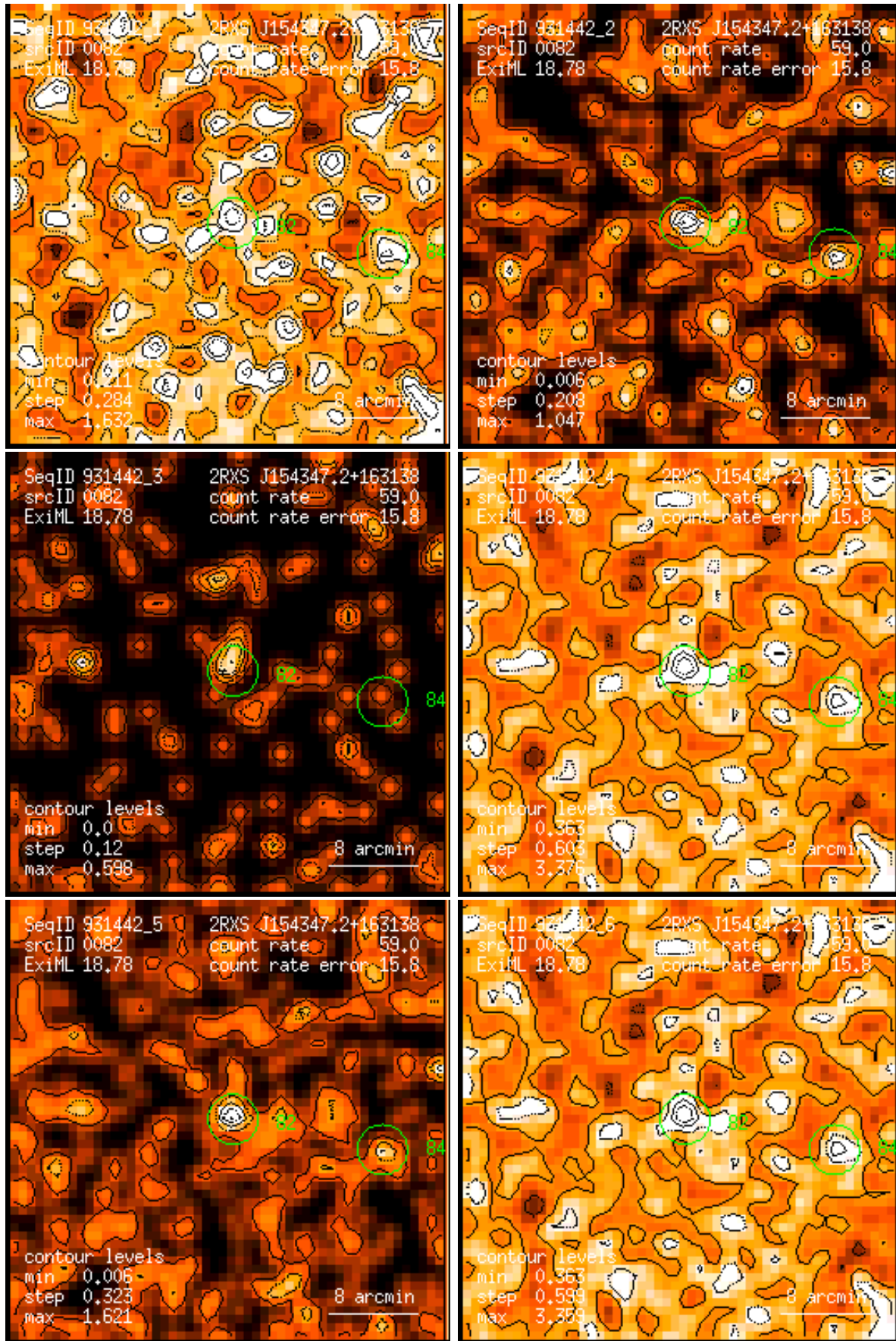
Figure 82: RASS 931442: detection 0082: band rate images, Gaussian filter: (1) PSPC channels 11 – 41, (2) 52 – 90, (3) 91 – 201, (4) 11 – 235, (5) 52 – 201, (6) 11 – 201. Broad band rates in counts/ks. Band rate contour levels in counts/ks/arcmin 2 .
