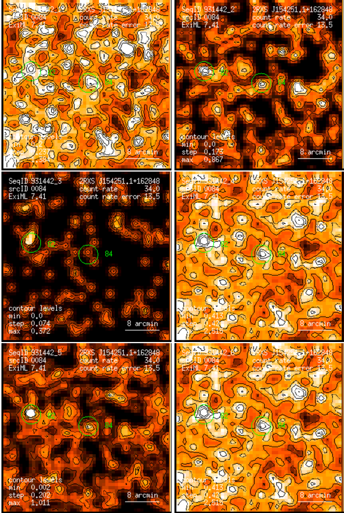
Figure 84: RASS 931442: detection 0084: band rate images, Gaussian filter: (1) PSPC channels 11 – 41, (2) 52 – 90, (3) 91 – 201, (4) 11 – 235, (5) 52 – 201, (6) 11 – 201. Broad band rates in counts/ks. Band rate contour levels in counts/ks/arcmin 2 .
