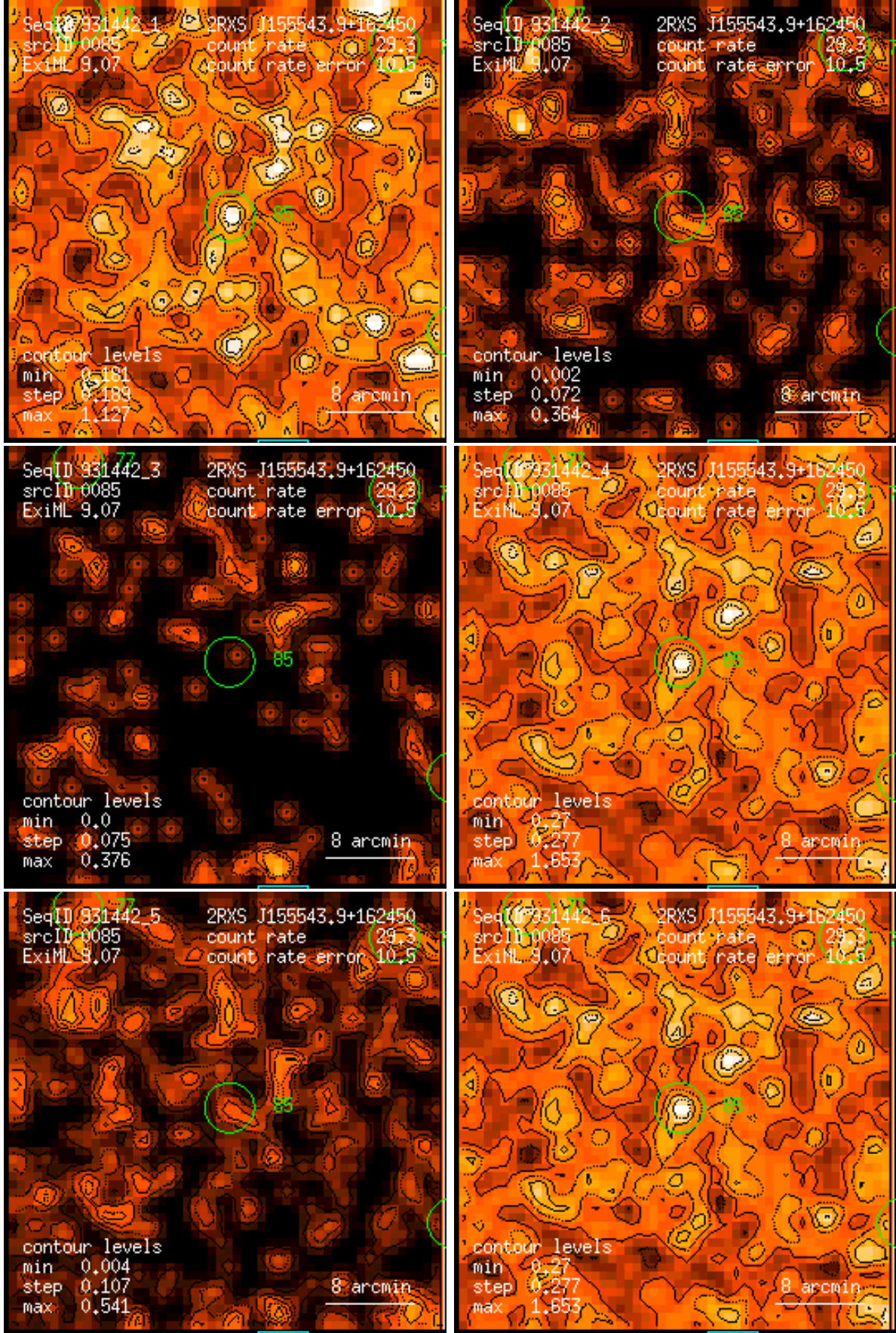
Figure 85: RASS 931442: detection 0085: band rate images, Gaussian filter: (1) PSPC channels 11 – 41, (2) 52 – 90, (3) 91 – 201, (4) 11 – 235, (5) 52 – 201, (6) 11 – 201. Broad band rates in counts/ks. Band rate contour levels in counts/ks/arcmin 2 .
