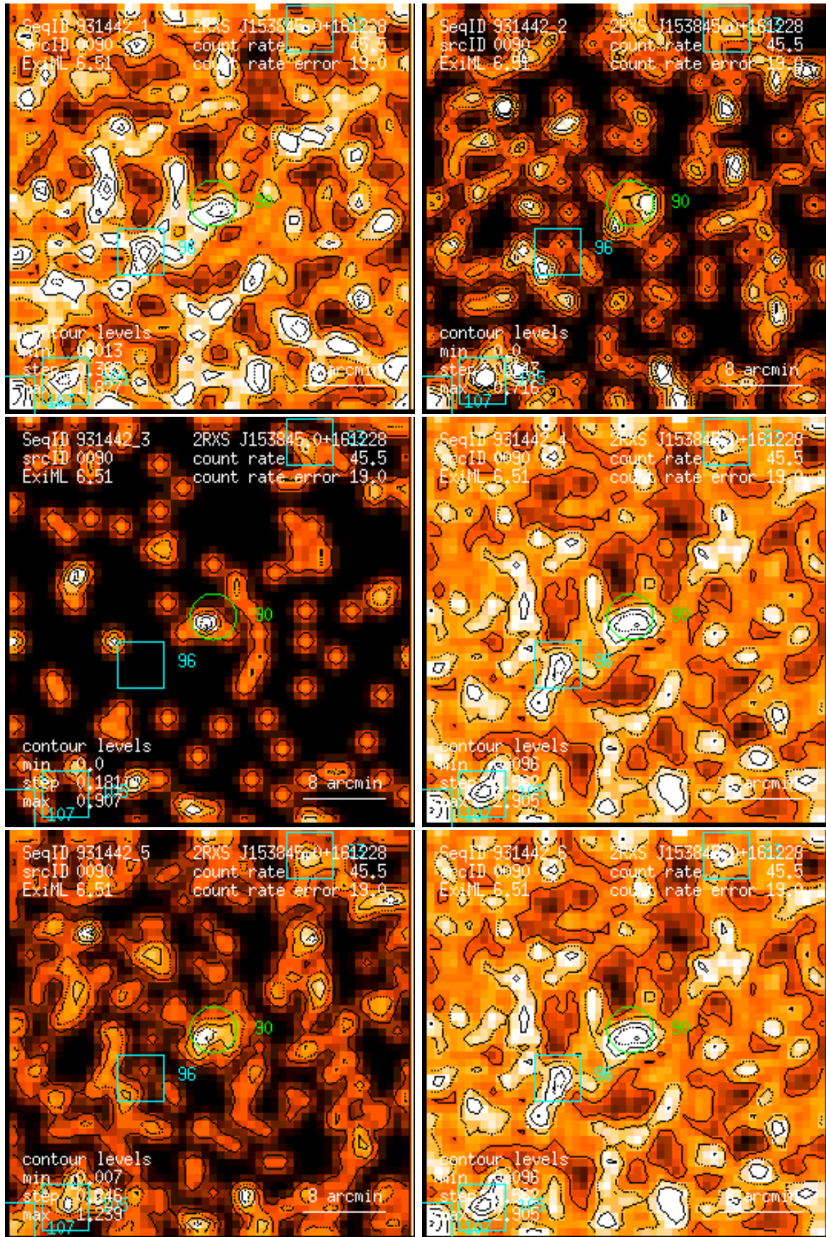
Figure 90: RASS 931442: detection 0090: band rate images, Gaussian filter: (1) PSPC channels 11 – 41, (2) 52 – 90, (3) 91 – 201, (4) 11 – 235, (5) 52 – 201, (6) 11 – 201. Broad band rates in counts/ks. Band rate contour levels in counts/ks/arcmin 2 .
