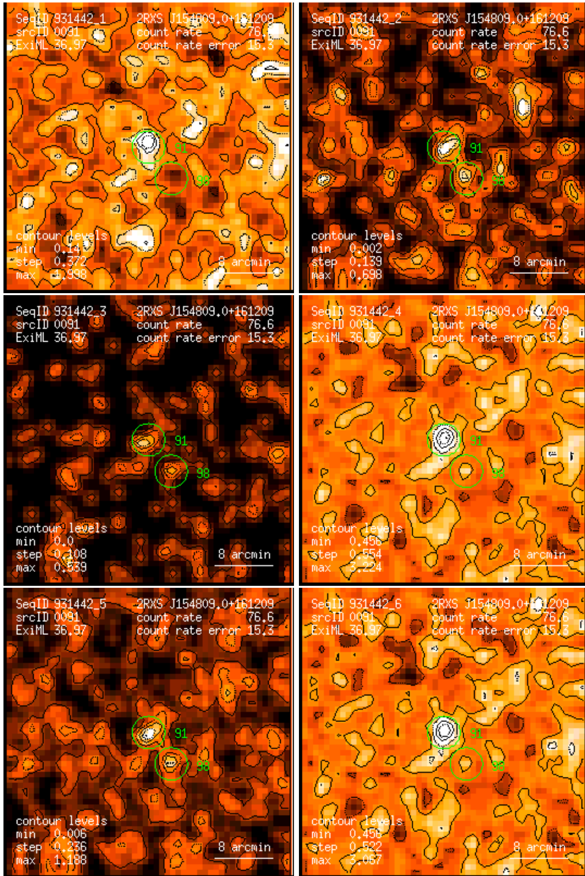
Figure 91: RASS 931442: detection 0091: band rate images, Gaussian filter: (1) PSPC channels 11 – 41, (2) 52 – 90, (3) 91 – 201, (4) 11 – 235, (5) 52 – 201, (6) 11 – 201. Broad band rates in counts/ks. Band rate contour levels in counts/ks/arcmin 2 .
