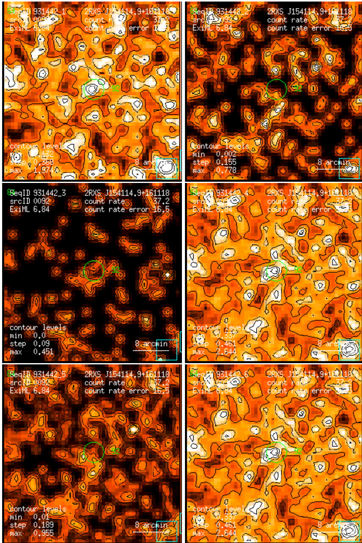
Figure 92: RASS 931442: detection 0092: band rate images, Gaussian filter: (1) PSPC channels 11 – 41, (2) 52 – 90, (3) 91 – 201, (4) 11 – 235, (5) 52 – 201, (6) 11 – 201. Broad band rates in counts/ks. Band rate contour levels in counts/ks/arcmin 2 .
