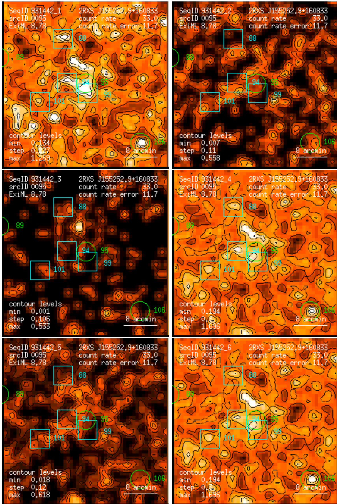
Figure 95: RASS 931442: detection 0095: band rate images, Gaussian filter: (1) PSPC channels 11 – 41, (2) 52 – 90, (3) 91 – 201, (4) 11 – 235, (5) 52 – 201, (6) 11 – 201. Broad band rates in counts/ks. Band rate contour levels in counts/ks/arcmin 2 .
