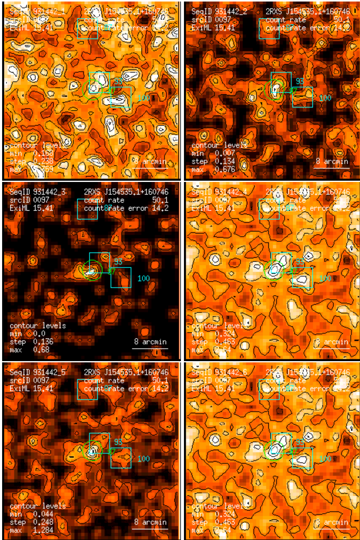
Figure 97: RASS 931442: detection 0097: band rate images, Gaussian filter: (1) PSPC channels 11 – 41, (2) 52 – 90, (3) 91 – 201, (4) 11 – 235, (5) 52 – 201, (6) 11 – 201. Broad band rates in counts/ks. Band rate contour levels in counts/ks/arcmin 2 .
