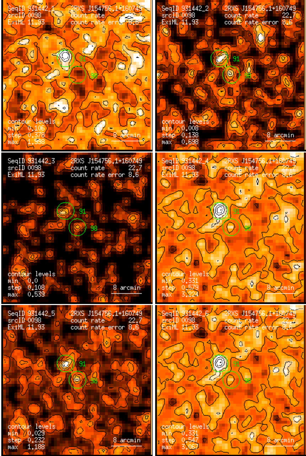
Figure 98: RASS 931442: detection 0098: band rate images, Gaussian filter: (1) PSPC channels 11 – 41, (2) 52 – 90, (3) 91 – 201, (4) 11 – 235, (5) 52 – 201, (6) 11 – 201. Broad band rates in counts/ks. Band rate contour levels in counts/ks/arcmin 2 .
