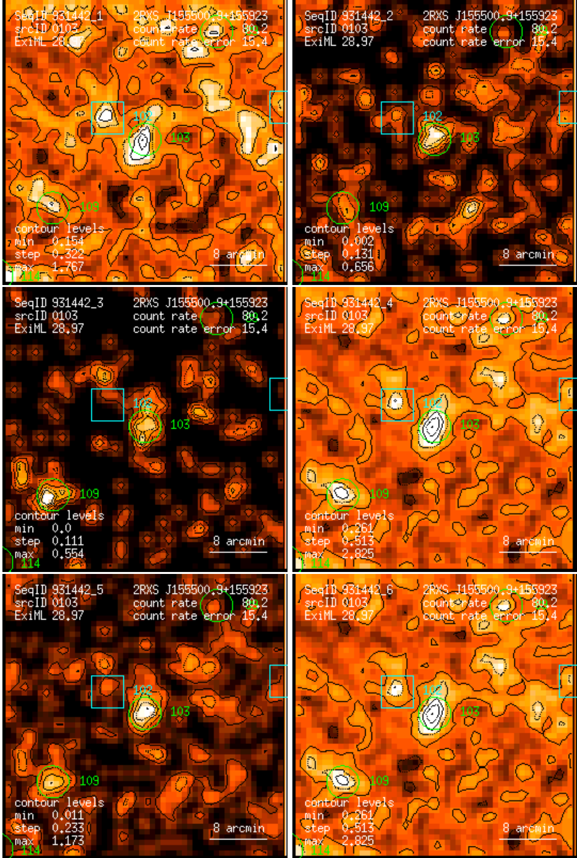
Figure 103: RASS 931442: detection 0103: band rate images, Gaussian filter: (1) PSPC channels 11 – 41, (2) 52 – 90, (3) 91 – 201, (4) 11 – 235, (5) 52 – 201, (6) 11 – 201. Broad band rates in counts/ks. Band rate contour levels in counts/ks/arcmin 2 .
