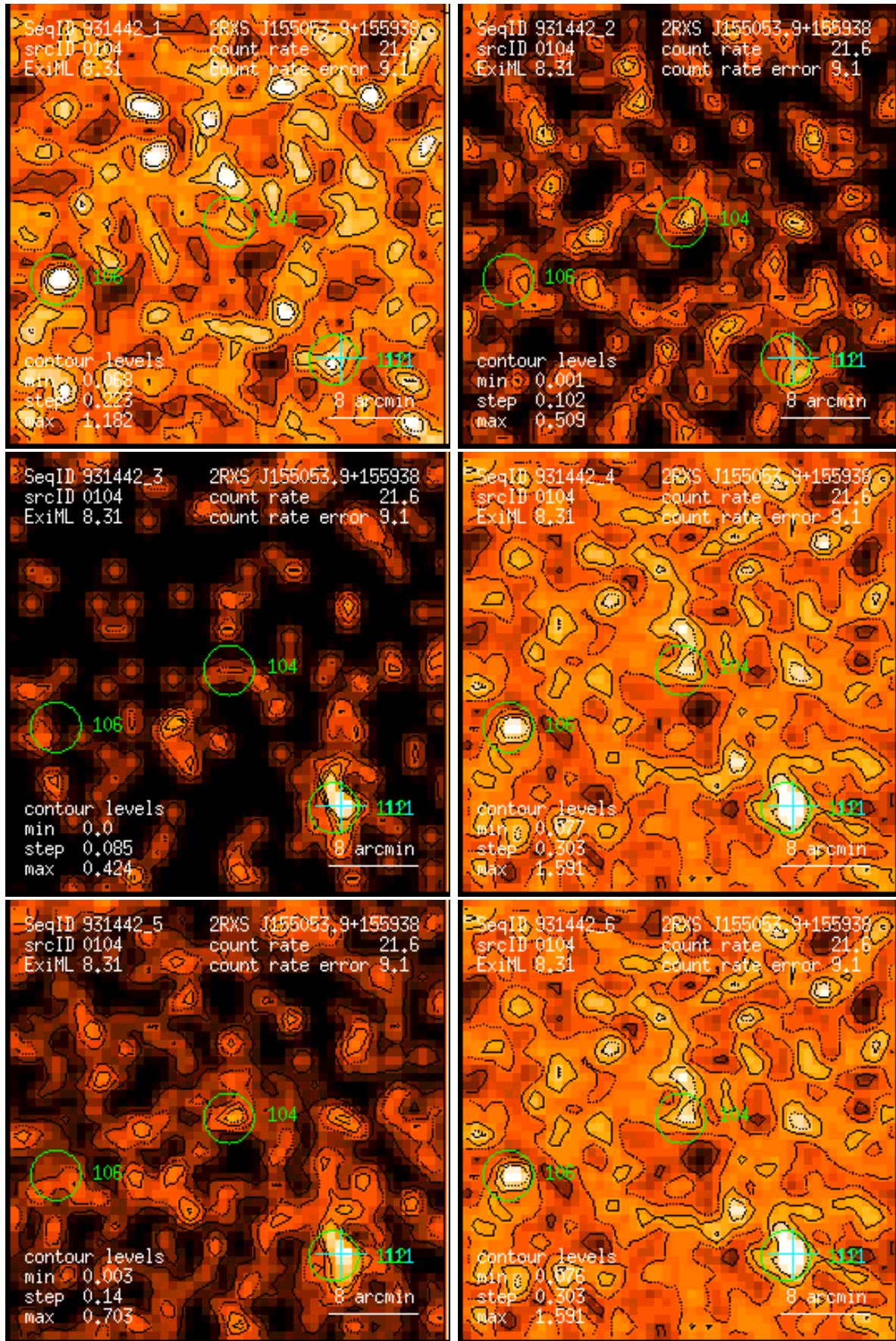
Figure 104: RASS 931442: detection 0104: band rate images, Gaussian filter: (1) PSPC channels 11 – 41, (2) 52 – 90, (3) 91 – 201, (4) 11 – 235, (5) 52 – 201, (6) 11 – 201. Broad band rates in counts/ks. Band rate contour levels in counts/ks/arcmin 2 .
