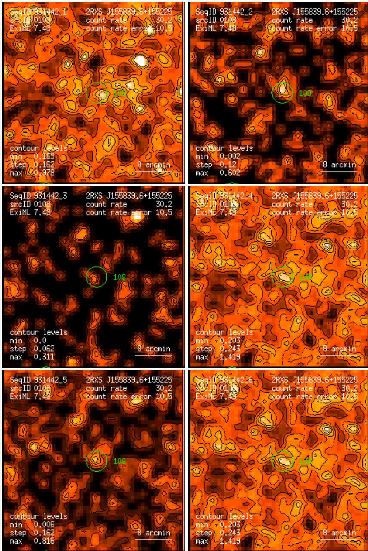
Figure 108: RASS 931442: detection 0108: band rate images, Gaussian filter: (1) PSPC channels 11 – 41, (2) 52 – 90, (3) 91 – 201, (4) 11 – 235, (5) 52 – 201, (6) 11 – 201. Broad band rates in counts/ks. Band rate contour levels in counts/ks/arcmin 2 .
