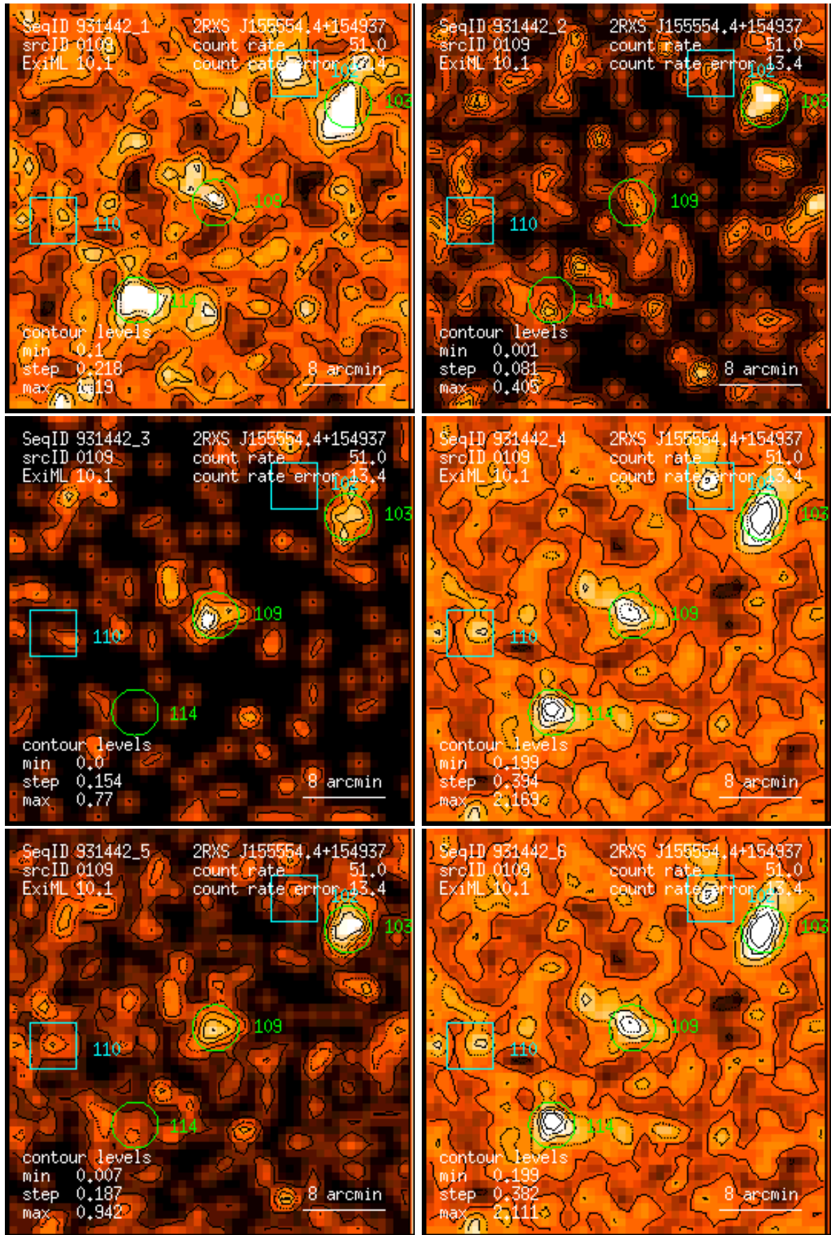
Figure 109: RASS 931442: detection 0109: band rate images, Gaussian filter: (1) PSPC channels 11 – 41, (2) 52 – 90, (3) 91 – 201, (4) 11 – 235, (5) 52 – 201, (6) 11 – 201. Broad band rates in counts/ks. Band rate contour levels in counts/ks/arcmin 2 .
