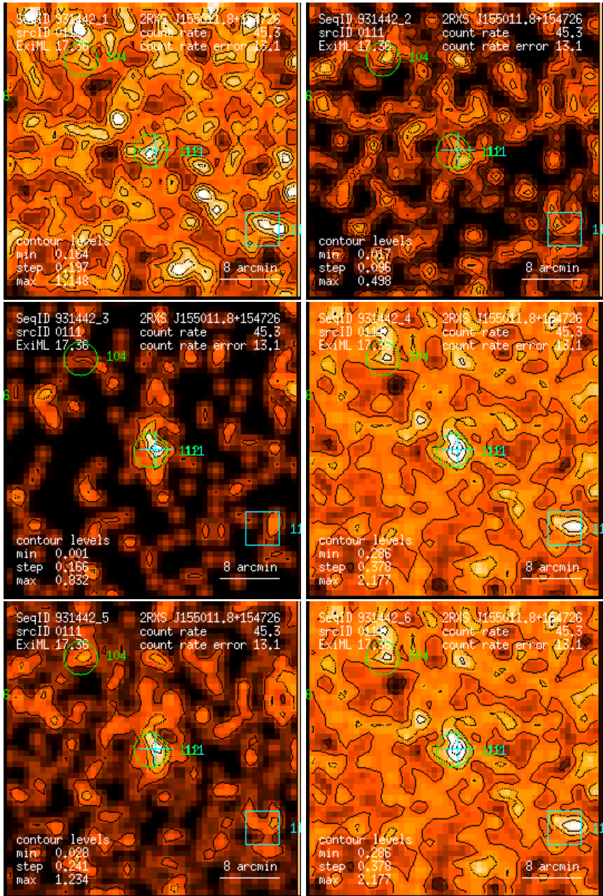
Figure 111: RASS 931442: detection 0111: band rate images, Gaussian filter: (1) PSPC channels 11 – 41, (2) 52 – 90, (3) 91 – 201, (4) 11 – 235, (5) 52 – 201, (6) 11 – 201. Broad band rates in counts/ks. Band rate contour levels in counts/ks/arcmin 2 .
