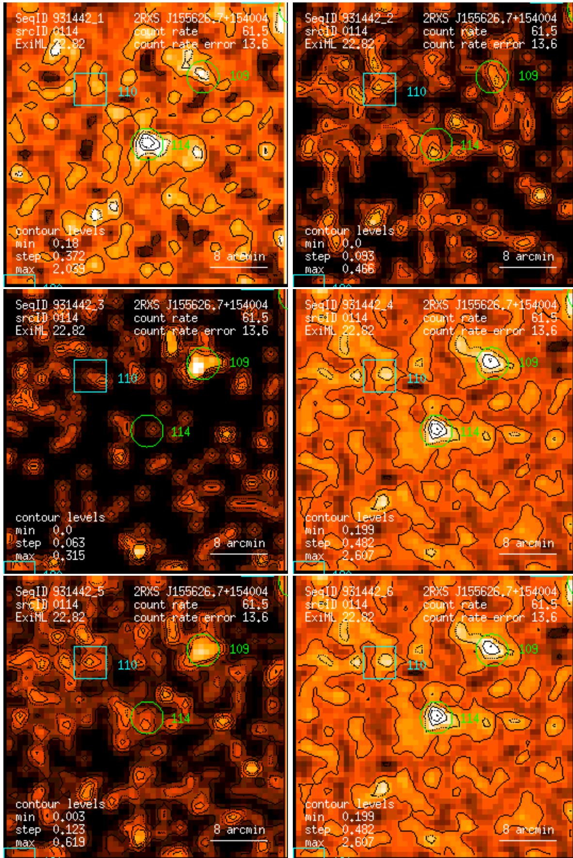
Figure 114: RASS 931442: detection 0114: band rate images, Gaussian filter: (1) PSPC channels 11 – 41, (2) 52 – 90, (3) 91 – 201, (4) 11 – 235, (5) 52 – 201, (6) 11 – 201. Broad band rates in counts/ks. Band rate contour levels in counts/ks/arcmin 2 .
