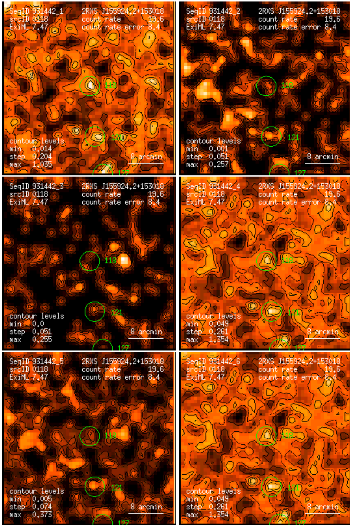
Figure 118: RASS 931442: detection 0118: band rate images, Gaussian filter: (1) PSPC channels 11 – 41, (2) 52 – 90, (3) 91 – 201, (4) 11 – 235, (5) 52 – 201, (6) 11 – 201. Broad band rates in counts/ks. Band rate contour levels in counts/ks/arcmin 2 .
