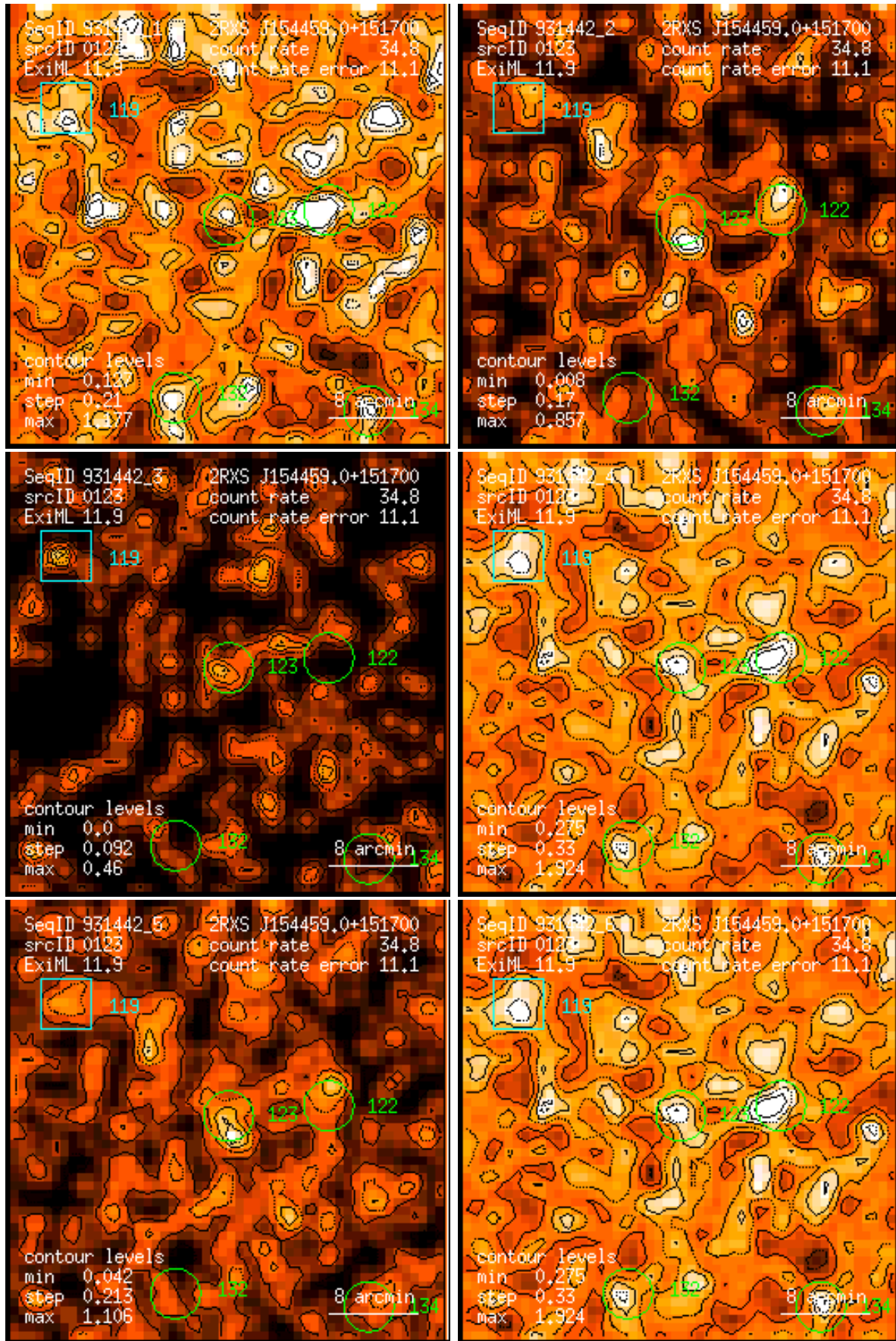
Figure 123: RASS 931442: detection 0123: band rate images, Gaussian filter: (1) PSPC channels 11 – 41, (2) 52 – 90, (3) 91 – 201, (4) 11 – 235, (5) 52 – 201, (6) 11 – 201. Broad band rates in counts/ks. Band rate contour levels in counts/ks/arcmin 2 .
