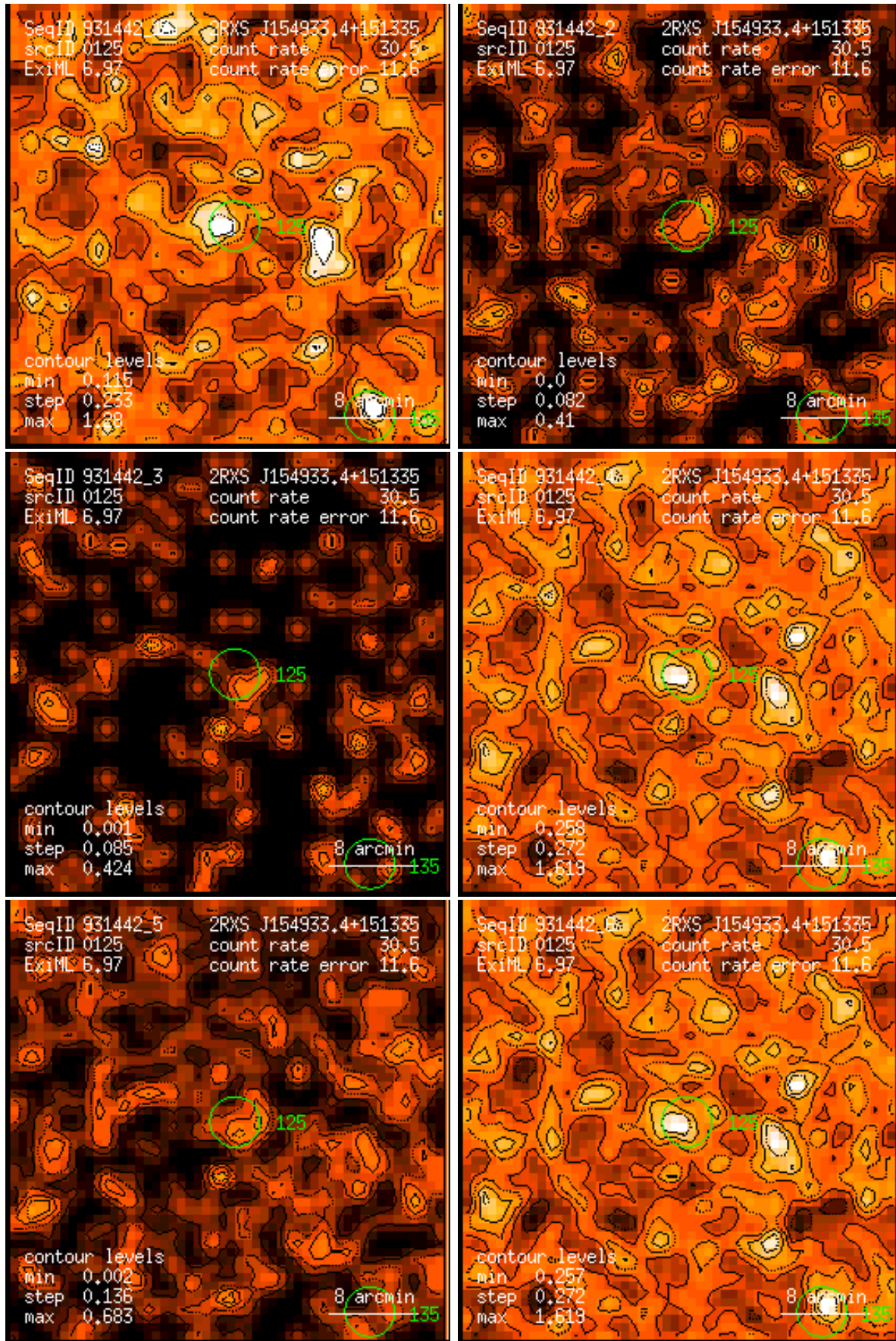
Figure 125: RASS 931442: detection 0125: band rate images, Gaussian filter: (1) PSPC channels 11 – 41, (2) 52 – 90, (3) 91 – 201, (4) 11 – 235, (5) 52 – 201, (6) 11 – 201. Broad band rates in counts/ks. Band rate contour levels in counts/ks/arcmin 2 .
