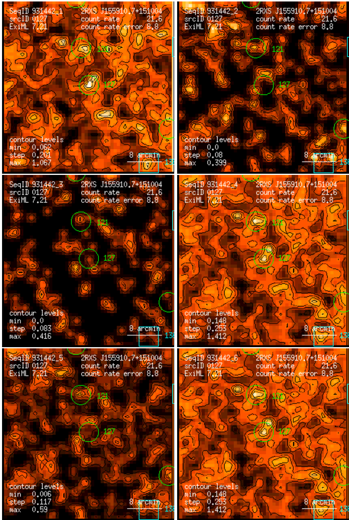
Figure 127: RASS 931442: detection 0127: band rate images, Gaussian filter: (1) PSPC channels 11 – 41, (2) 52 – 90, (3) 91 – 201, (4) 11 – 235, (5) 52 – 201, (6) 11 – 201. Broad band rates in counts/ks. Band rate contour levels in counts/ks/arcmin 2 .
