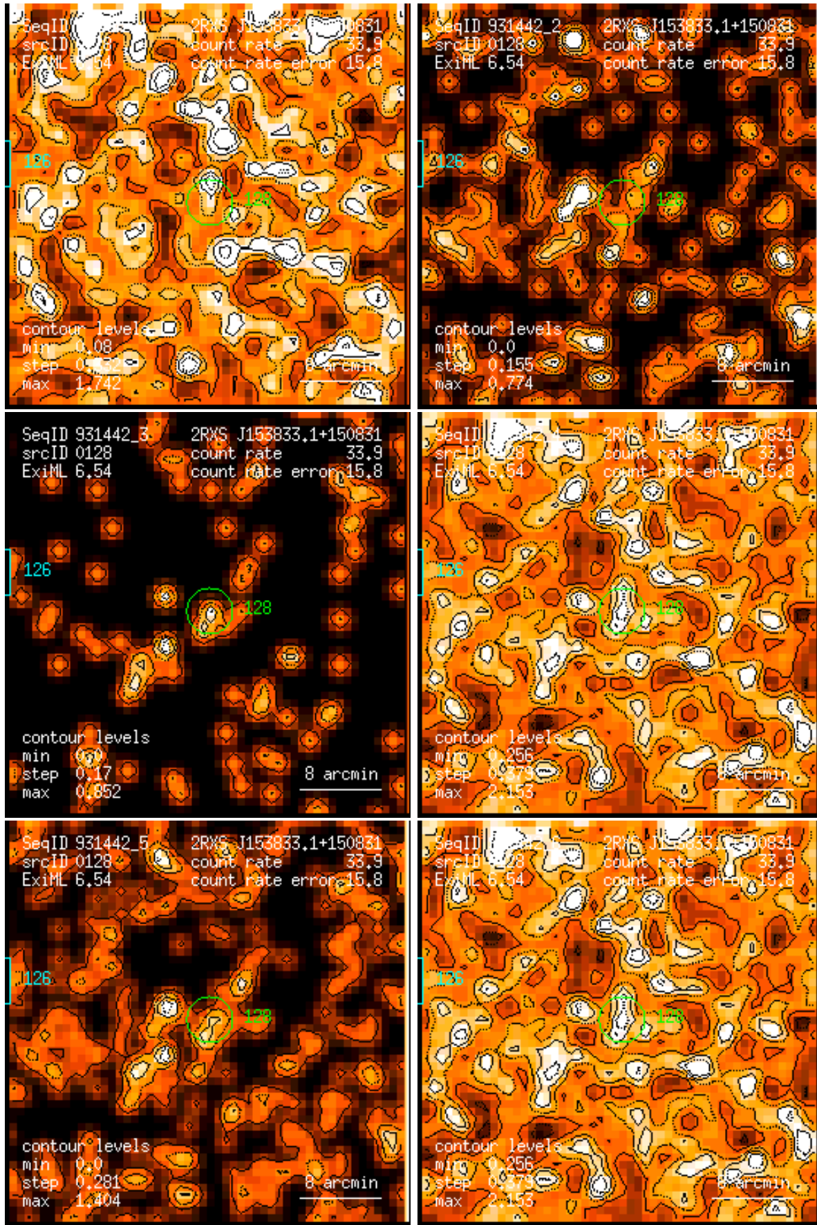
Figure 128: RASS 931442: detection 0128: band rate images, Gaussian filter: (1) PSPC channels 11 – 41, (2) 52 – 90, (3) 91 – 201, (4) 11 – 235, (5) 52 – 201, (6) 11 – 201. Broad band rates in counts/ks. Band rate contour levels in counts/ks/arcmin 2 .
