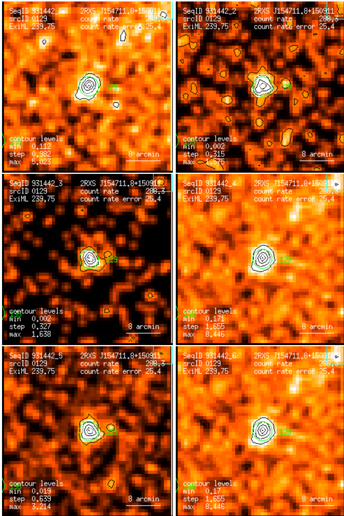
Figure 129: RASS 931442: detection 0129: band rate images, Gaussian filter: (1) PSPC channels 11 – 41, (2) 52 – 90, (3) 91 – 201, (4) 11 – 235, (5) 52 – 201, (6) 11 – 201. Broad band rates in counts/ks. Band rate contour levels in counts/ks/arcmin 2 .
