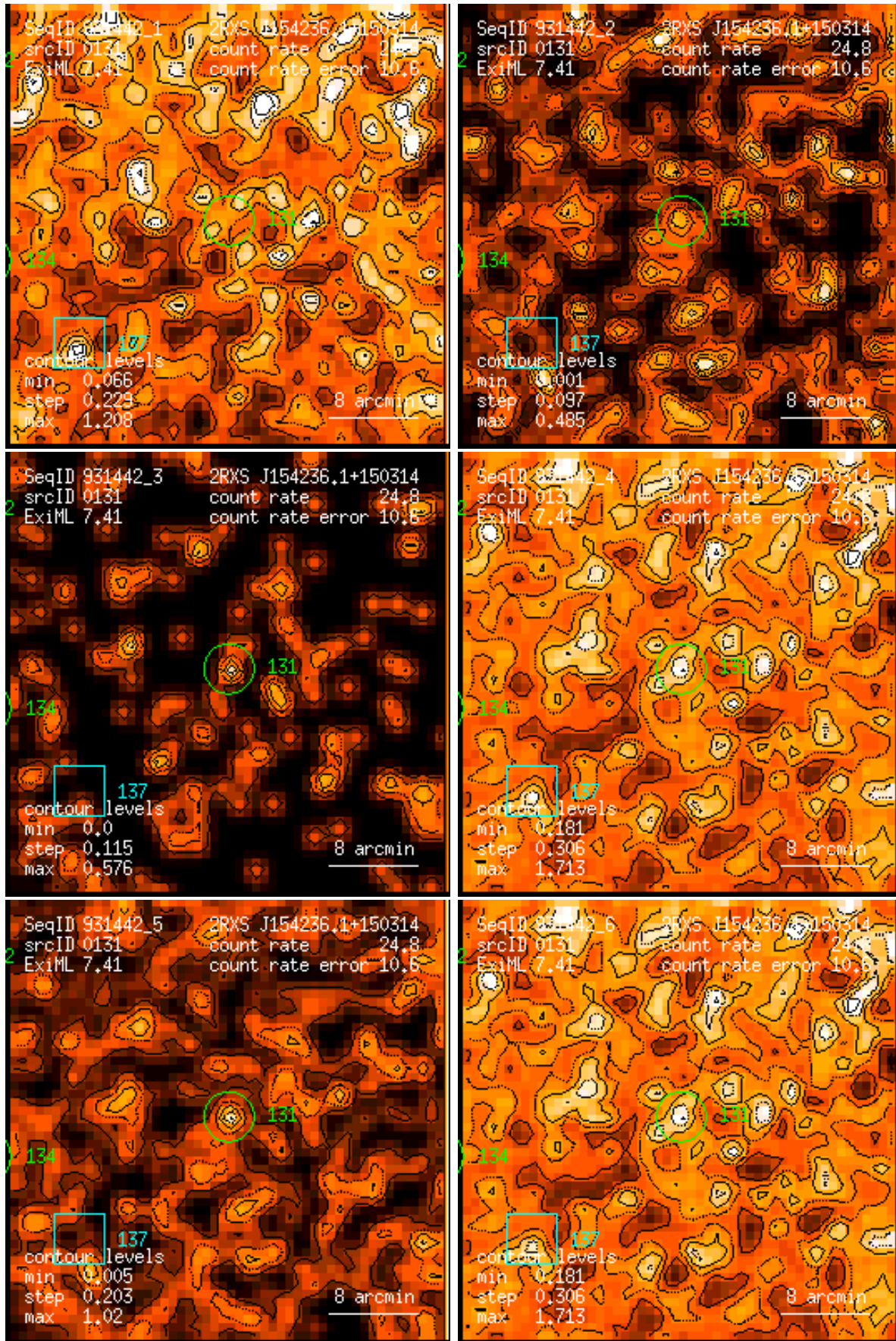
Figure 131: RASS 931442: detection 0131: band rate images, Gaussian filter: (1) PSPC channels 11 – 41, (2) 52 – 90, (3) 91 – 201, (4) 11 – 235, (5) 52 – 201, (6) 11 – 201. Broad band rates in counts/ks. Band rate contour levels in counts/ks/arcmin 2 .
