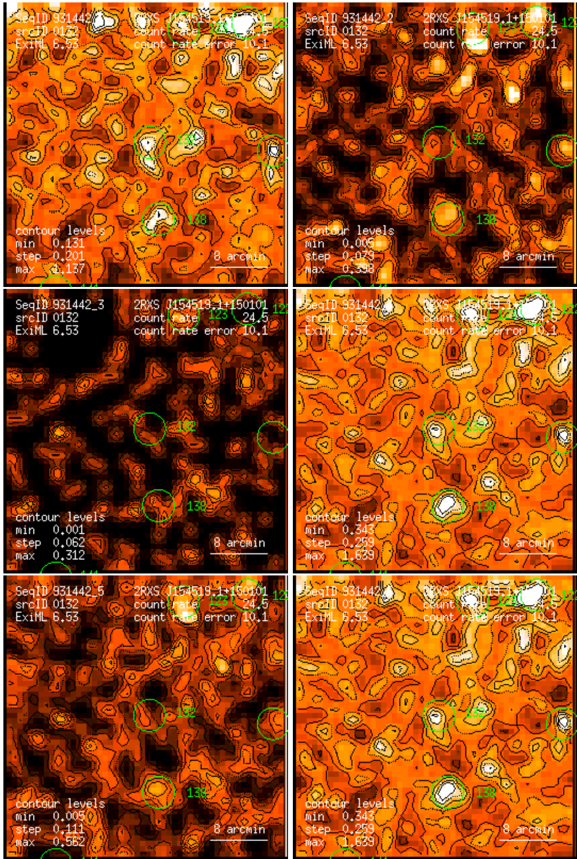
Figure 132: RASS 931442: detection 0132: band rate images, Gaussian filter: (1) PSPC channels 11 – 41, (2) 52 – 90, (3) 91 – 201, (4) 11 – 235, (5) 52 – 201, (6) 11 – 201. Broad band rates in counts/ks. Band rate contour levels in counts/ks/arcmin 2 .
