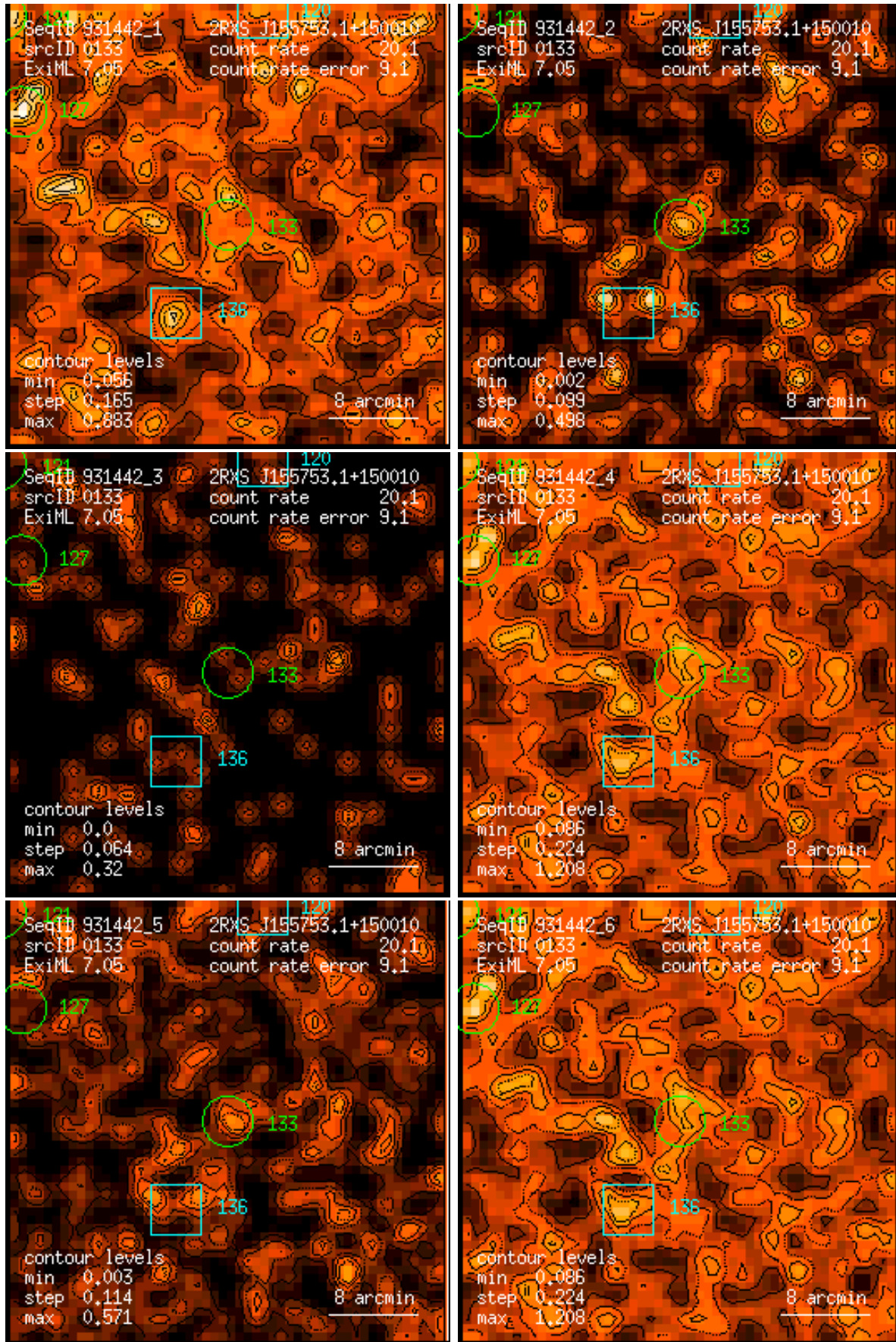
Figure 133: RASS 931442: detection 0133: band rate images, Gaussian filter: (1) PSPC channels 11 – 41, (2) 52 – 90, (3) 91 – 201, (4) 11 – 235, (5) 52 – 201, (6) 11 – 201. Broad band rates in counts/ks. Band rate contour levels in counts/ks/arcmin 2 .
