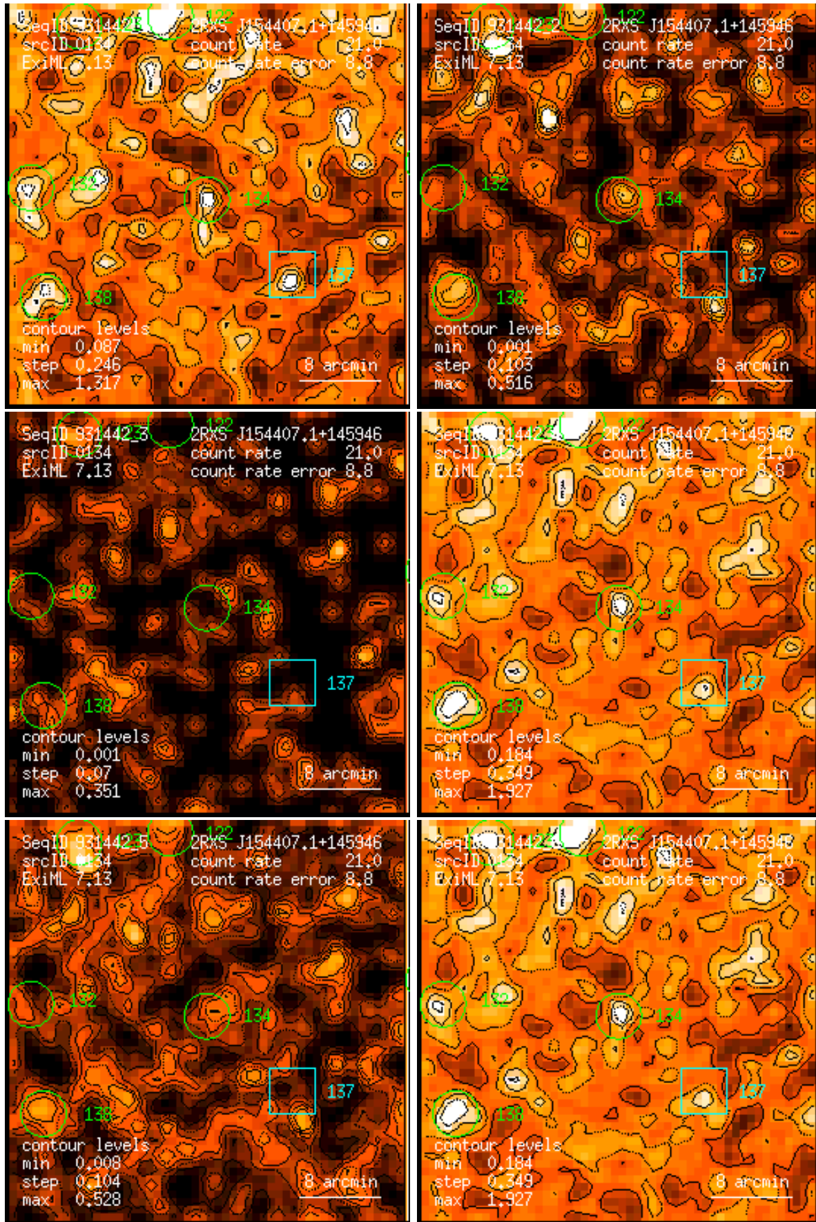
Figure 134: RASS 931442: detection 0134: band rate images, Gaussian filter: (1) PSPC channels 11 – 41, (2) 52 – 90, (3) 91 – 201, (4) 11 – 235, (5) 52 – 201, (6) 11 – 201. Broad band rates in counts/ks. Band rate contour levels in counts/ks/arcmin 2 .
