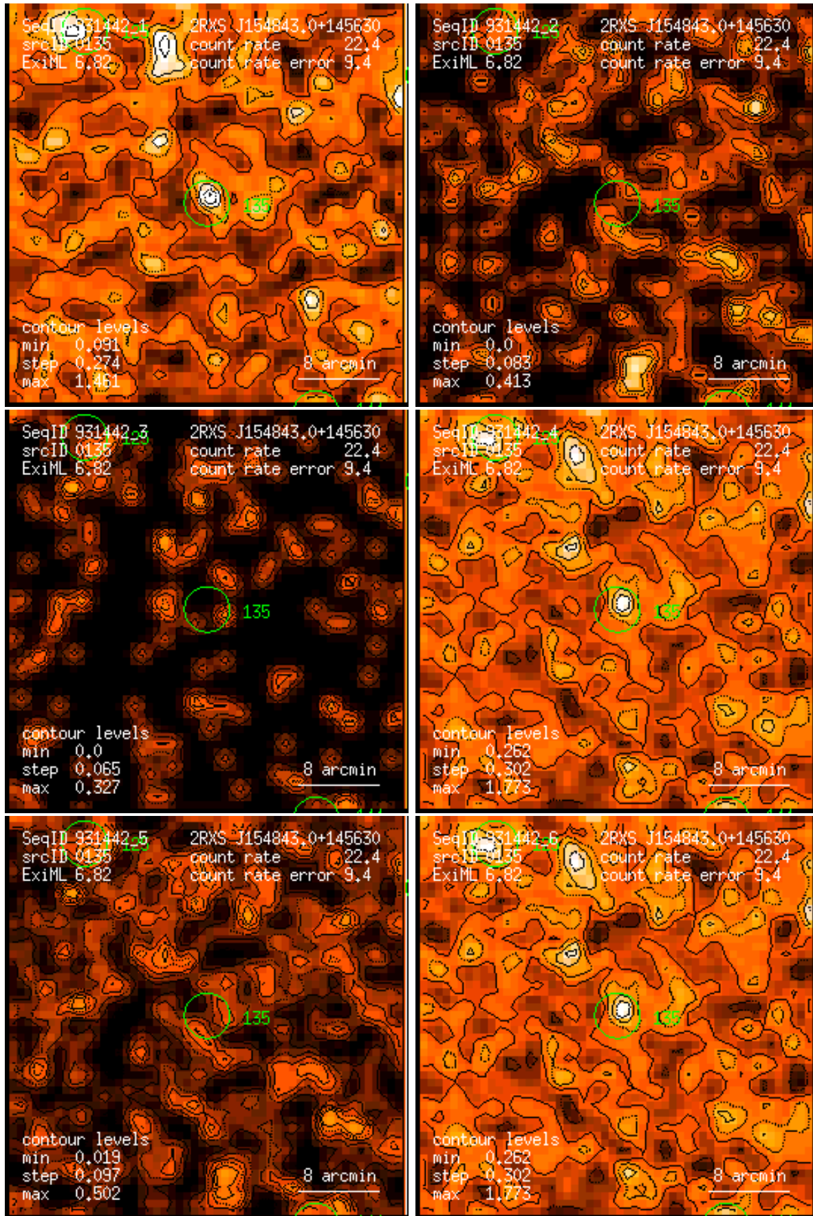
Figure 135: RASS 931442: detection 0135: band rate images, Gaussian filter: (1) PSPC channels 11 – 41, (2) 52 – 90, (3) 91 – 201, (4) 11 – 235, (5) 52 – 201, (6) 11 – 201. Broad band rates in counts/ks. Band rate contour levels in counts/ks/arcmin 2 .
