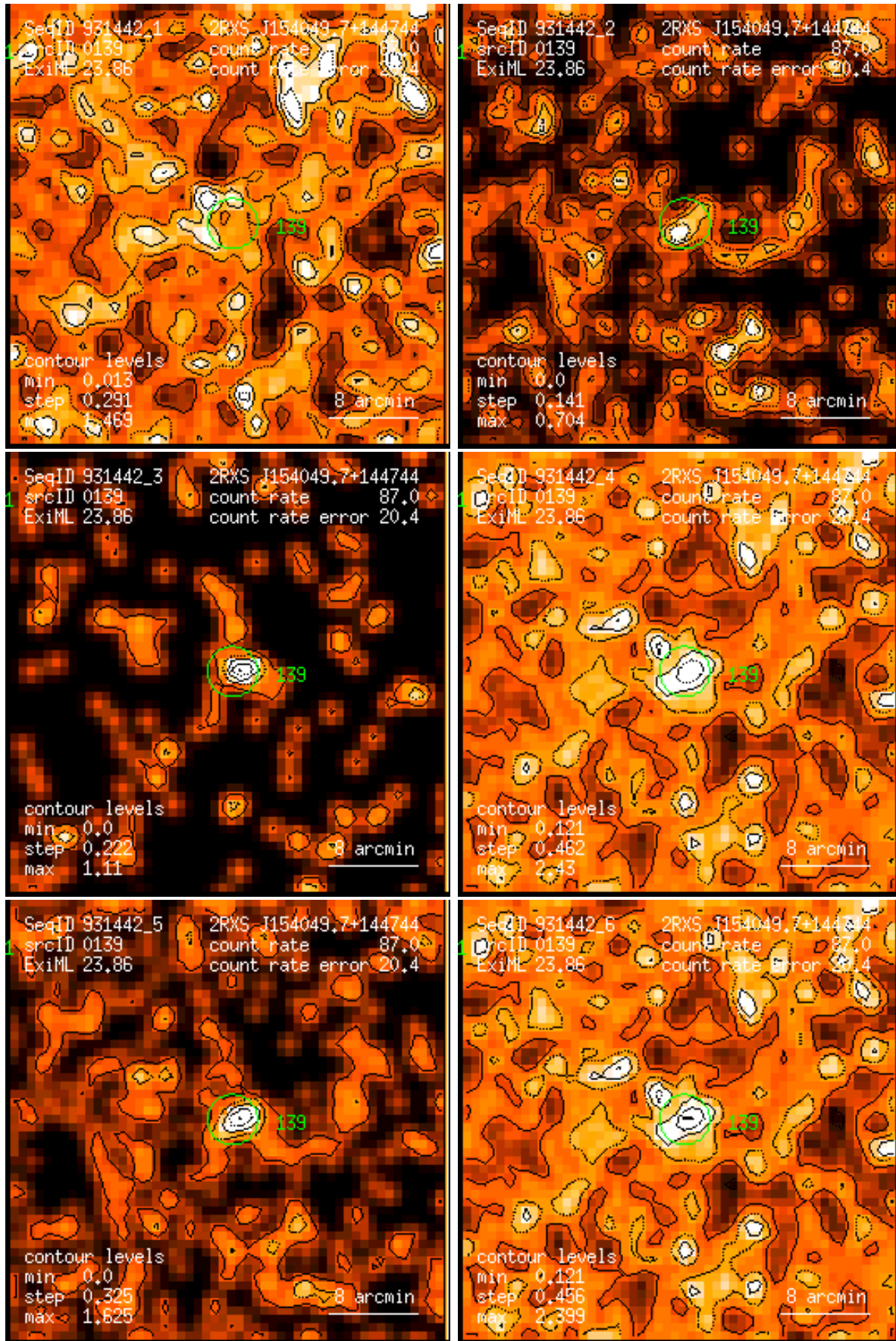
Figure 139: RASS 931442: detection 0139: band rate images, Gaussian filter: (1) PSPC channels 11 – 41, (2) 52 – 90, (3) 91 – 201, (4) 11 – 235, (5) 52 – 201, (6) 11 – 201. Broad band rates in counts/ks. Band rate contour levels in counts/ks/arcmin 2 .
