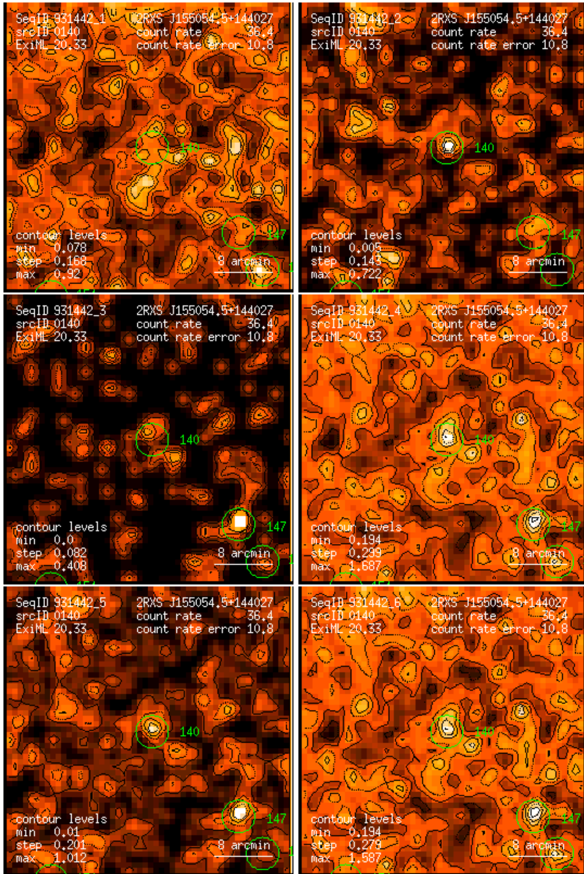
Figure 140: RASS 931442: detection 0140: band rate images, Gaussian filter: (1) PSPC channels 11 – 41, (2) 52 – 90, (3) 91 – 201, (4) 11 – 235, (5) 52 – 201, (6) 11 – 201. Broad band rates in counts/ks. Band rate contour levels in counts/ks/arcmin 2 .
