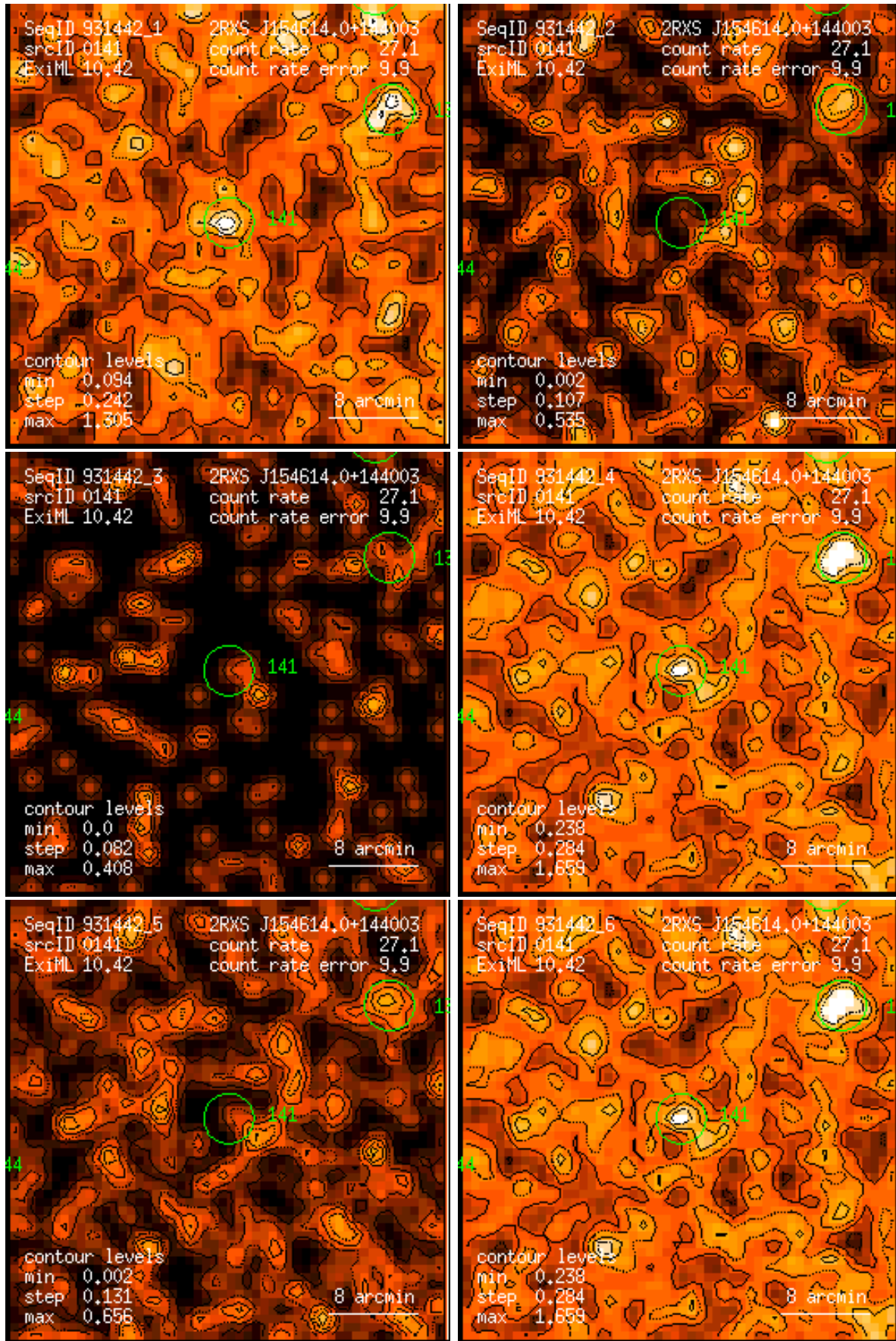
Figure 141: RASS 931442: detection 0141: band rate images, Gaussian filter: (1) PSPC channels 11 – 41, (2) 52 – 90, (3) 91 – 201, (4) 11 – 235, (5) 52 – 201, (6) 11 – 201. Broad band rates in counts/ks. Band rate contour levels in counts/ks/arcmin 2 .
