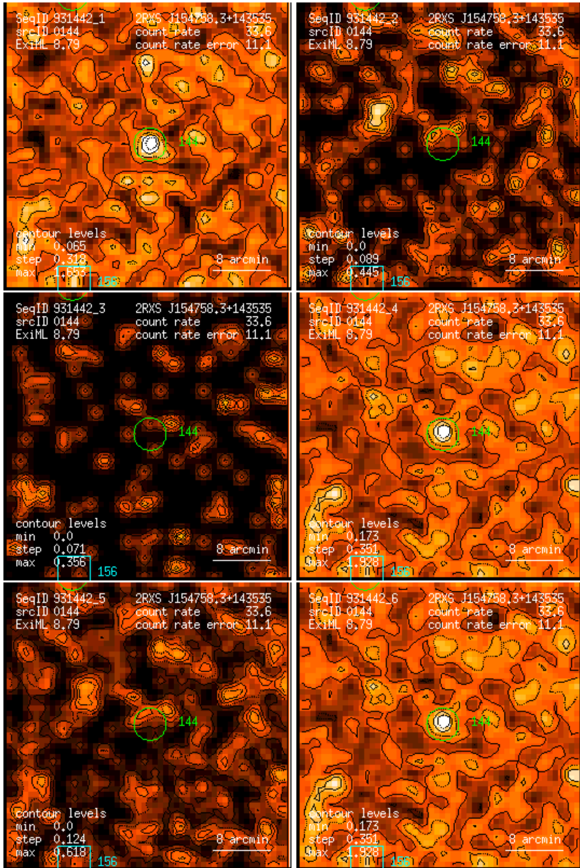
Figure 144: RASS 931442: detection 0144: band rate images, Gaussian filter: (1) PSPC channels 11 – 41, (2) 52 – 90, (3) 91 – 201, (4) 11 – 235, (5) 52 – 201, (6) 11 – 201. Broad band rates in counts/ks. Band rate contour levels in counts/ks/arcmin 2 .
