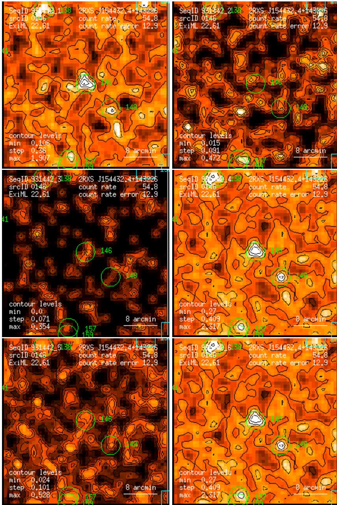
Figure 146: RASS 931442: detection 0146: band rate images, Gaussian filter: (1) PSPC channels 11 – 41, (2) 52 – 90, (3) 91 – 201, (4) 11 – 235, (5) 52 – 201, (6) 11 – 201. Broad band rates in counts/ks. Band rate contour levels in counts/ks/arcmin 2 .
