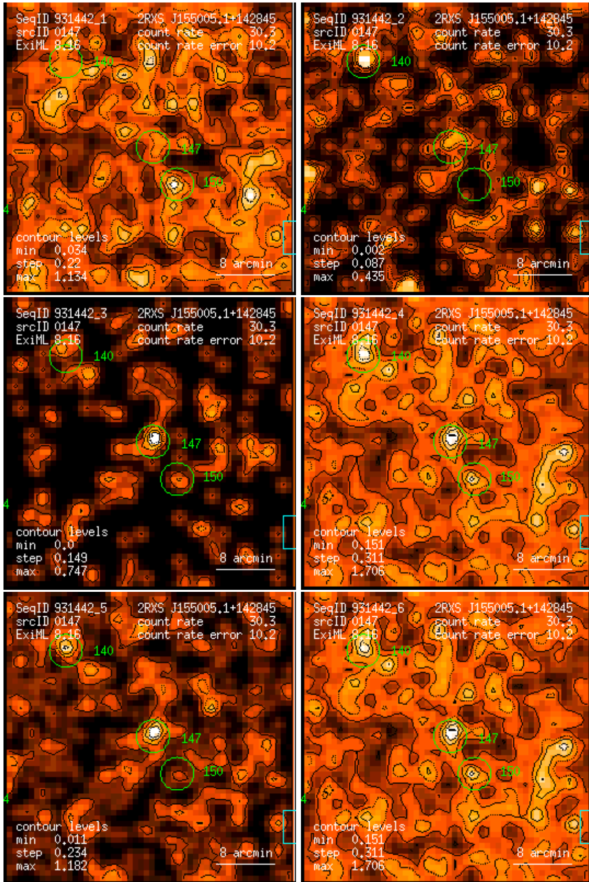
Figure 147: RASS 931442: detection 0147: band rate images, Gaussian filter: (1) PSPC channels 11 – 41, (2) 52 – 90, (3) 91 – 201, (4) 11 – 235, (5) 52 – 201, (6) 11 – 201. Broad band rates in counts/ks. Band rate contour levels in counts/ks/arcmin 2 .
