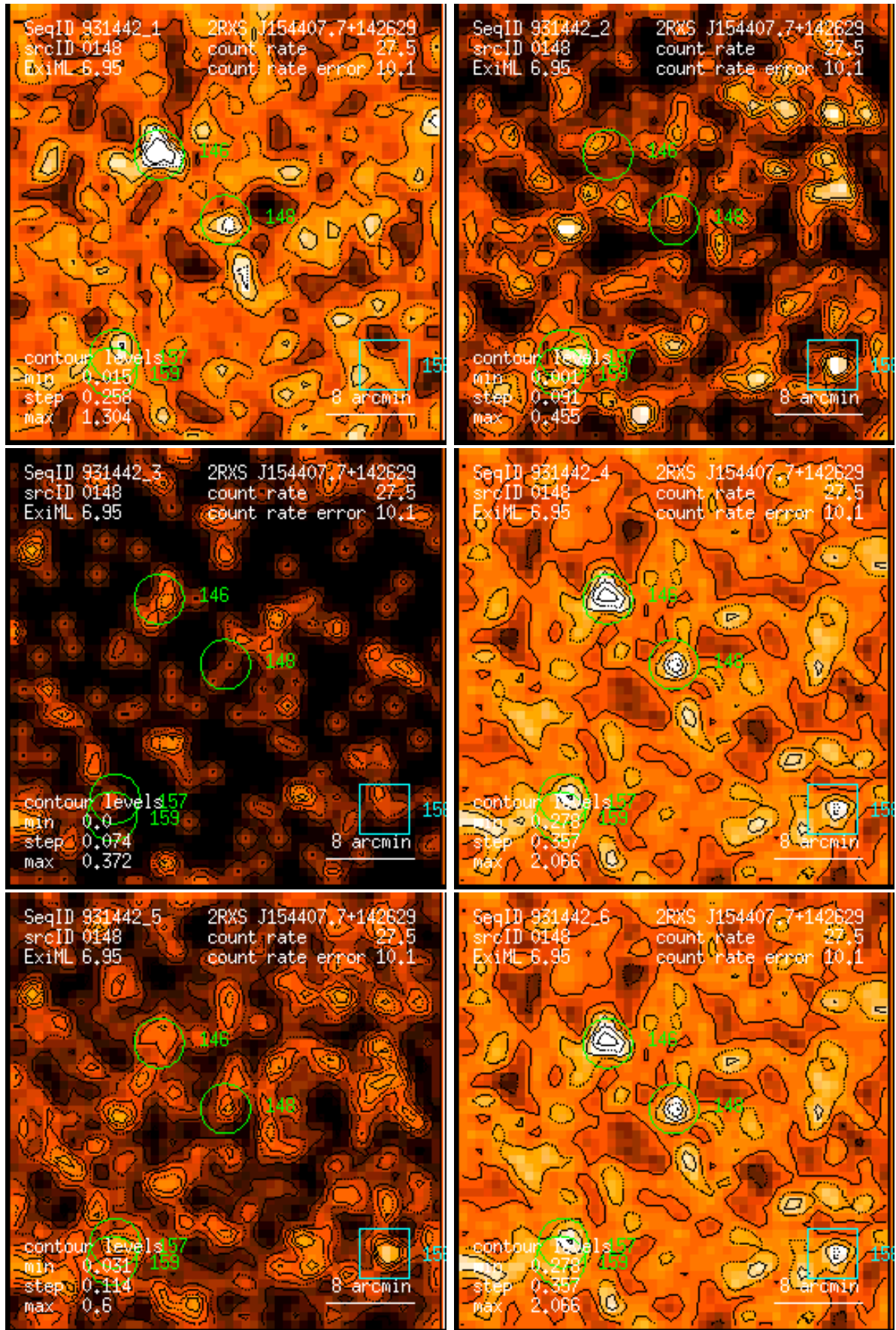
Figure 148: RASS 931442: detection 0148: band rate images, Gaussian filter: (1) PSPC channels 11 – 41, (2) 52 – 90, (3) 91 – 201, (4) 11 – 235, (5) 52 – 201, (6) 11 – 201. Broad band rates in counts/ks. Band rate contour levels in counts/ks/arcmin 2 .
