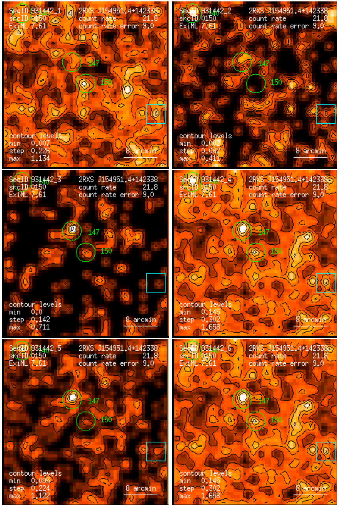
Figure 150: RASS 931442: detection 0150: band rate images, Gaussian filter: (1) PSPC channels 11 – 41, (2) 52 – 90, (3) 91 – 201, (4) 11 – 235, (5) 52 – 201, (6) 11 – 201. Broad band rates in counts/ks. Band rate contour levels in counts/ks/arcmin 2 .
