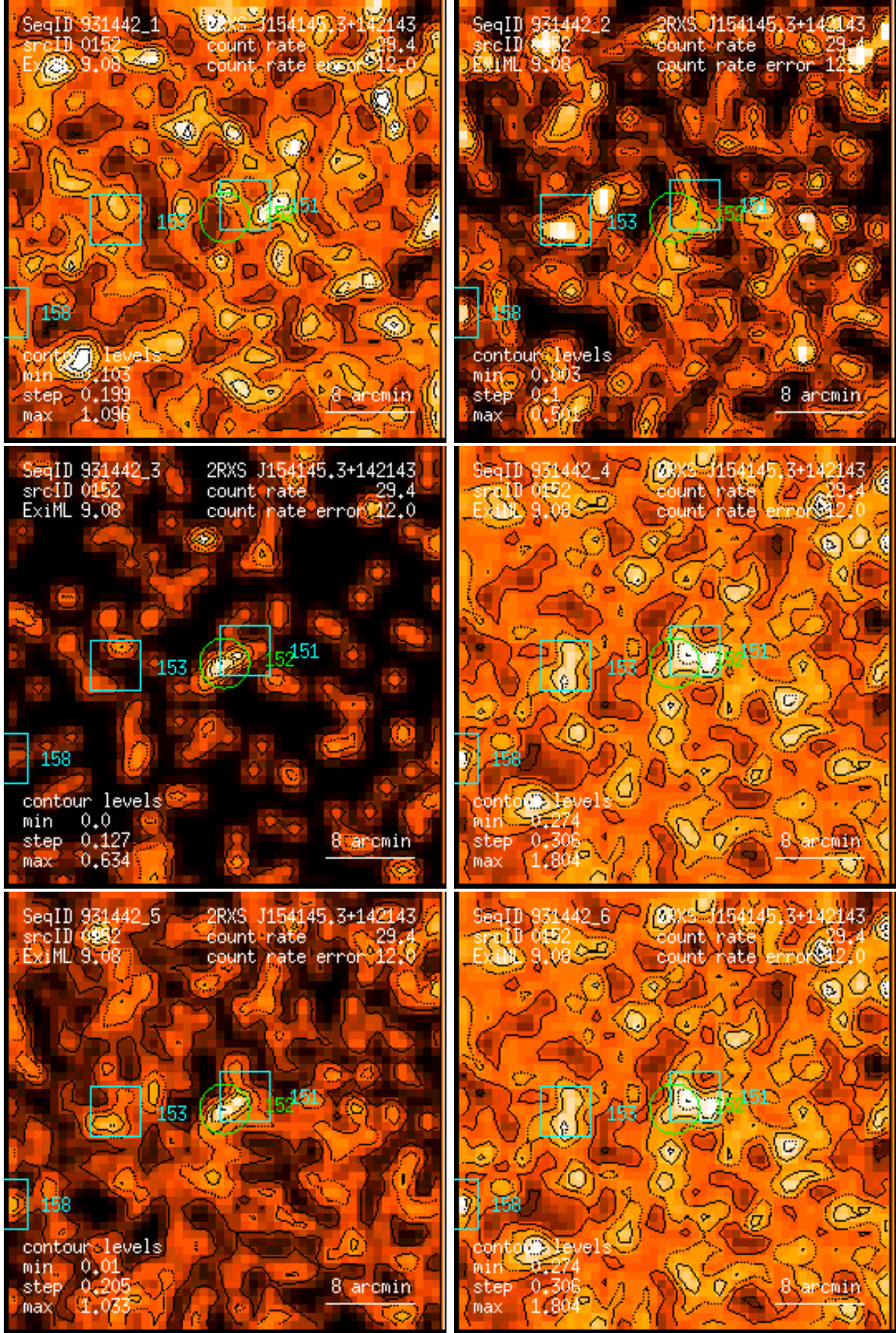
Figure 152: RASS 931442: detection 0152: band rate images, Gaussian filter: (1) PSPC channels 11 – 41, (2) 52 – 90, (3) 91 – 201, (4) 11 – 235, (5) 52 – 201, (6) 11 – 201. Broad band rates in counts/ks. Band rate contour levels in counts/ks/arcmin 2 .
