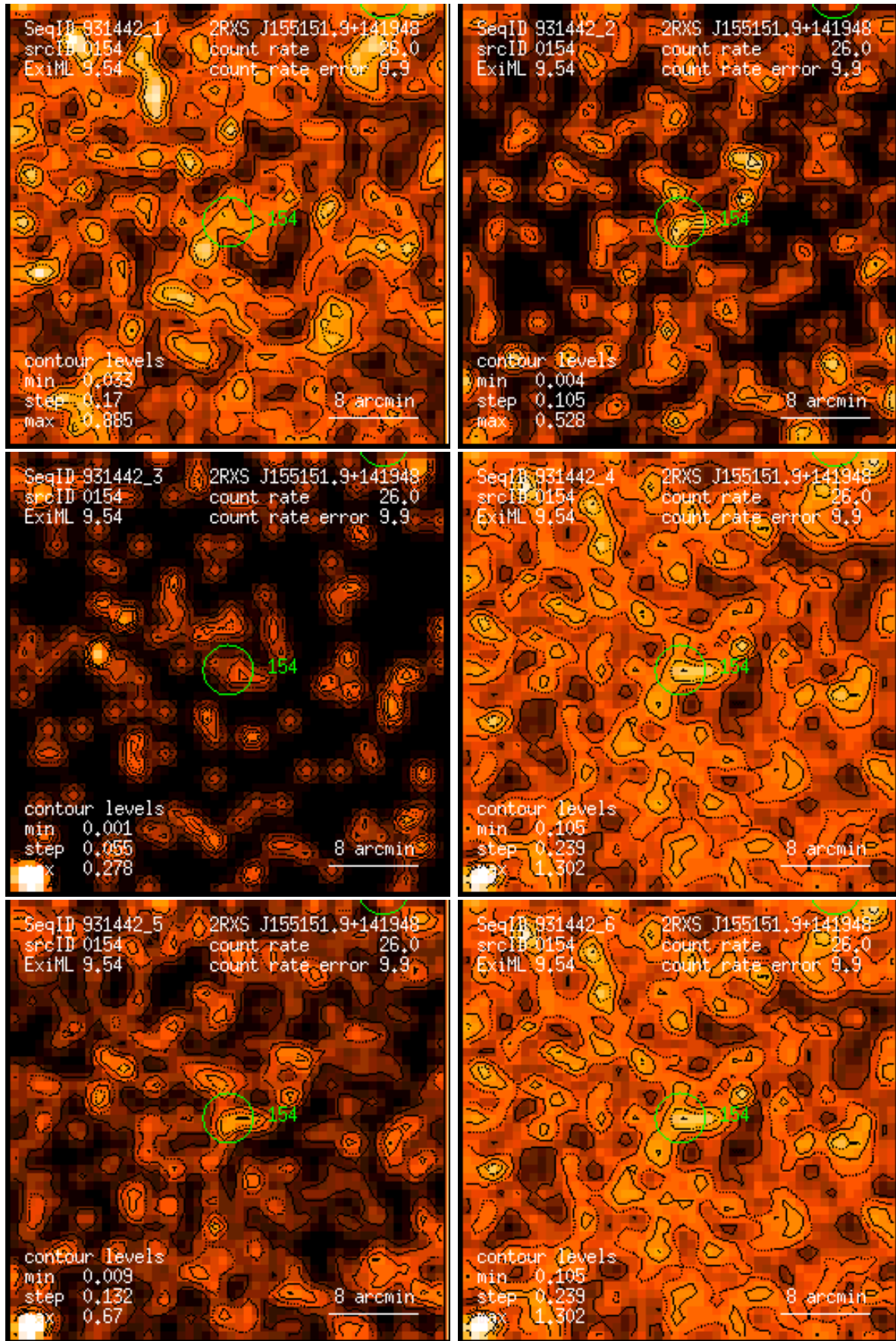
Figure 154: RASS 931442: detection 0154: band rate images, Gaussian filter: (1) PSPC channels 11 – 41, (2) 52 – 90, (3) 91 – 201, (4) 11 – 235, (5) 52 – 201, (6) 11 – 201. Broad band rates in counts/ks. Band rate contour levels in counts/ks/arcmin 2 .
